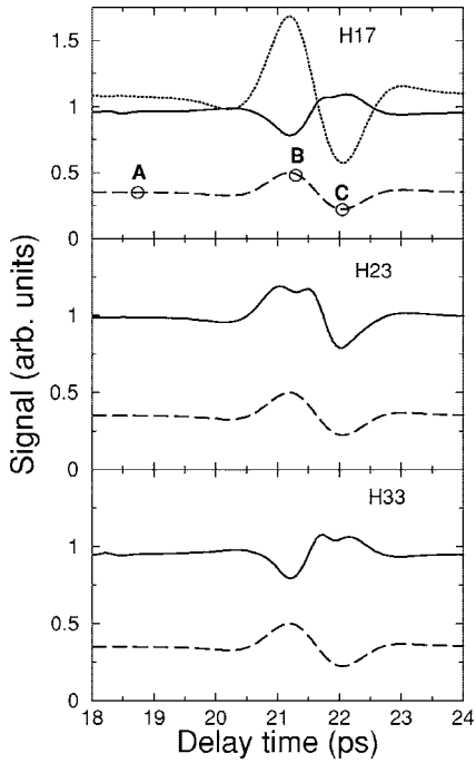
FIG. 3. Same as Fig. 2 but near half revival. On the top panel the ionization signal (dotted curve) is also shown.
