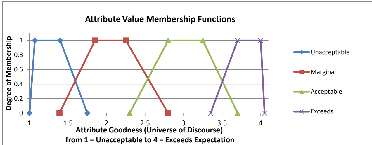
Figure 2. Fuzzy Attribute Value Membership Functions from RT-37
