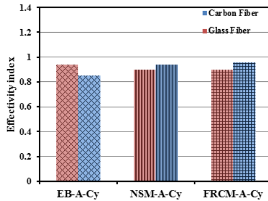
Figure 13. Effectivity index for different strengthening systems
