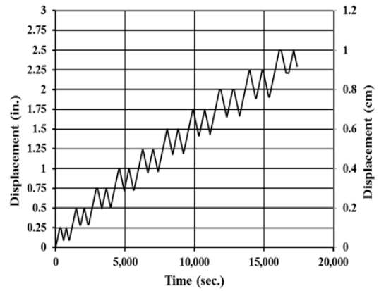
Figure 3. Loading protocol
