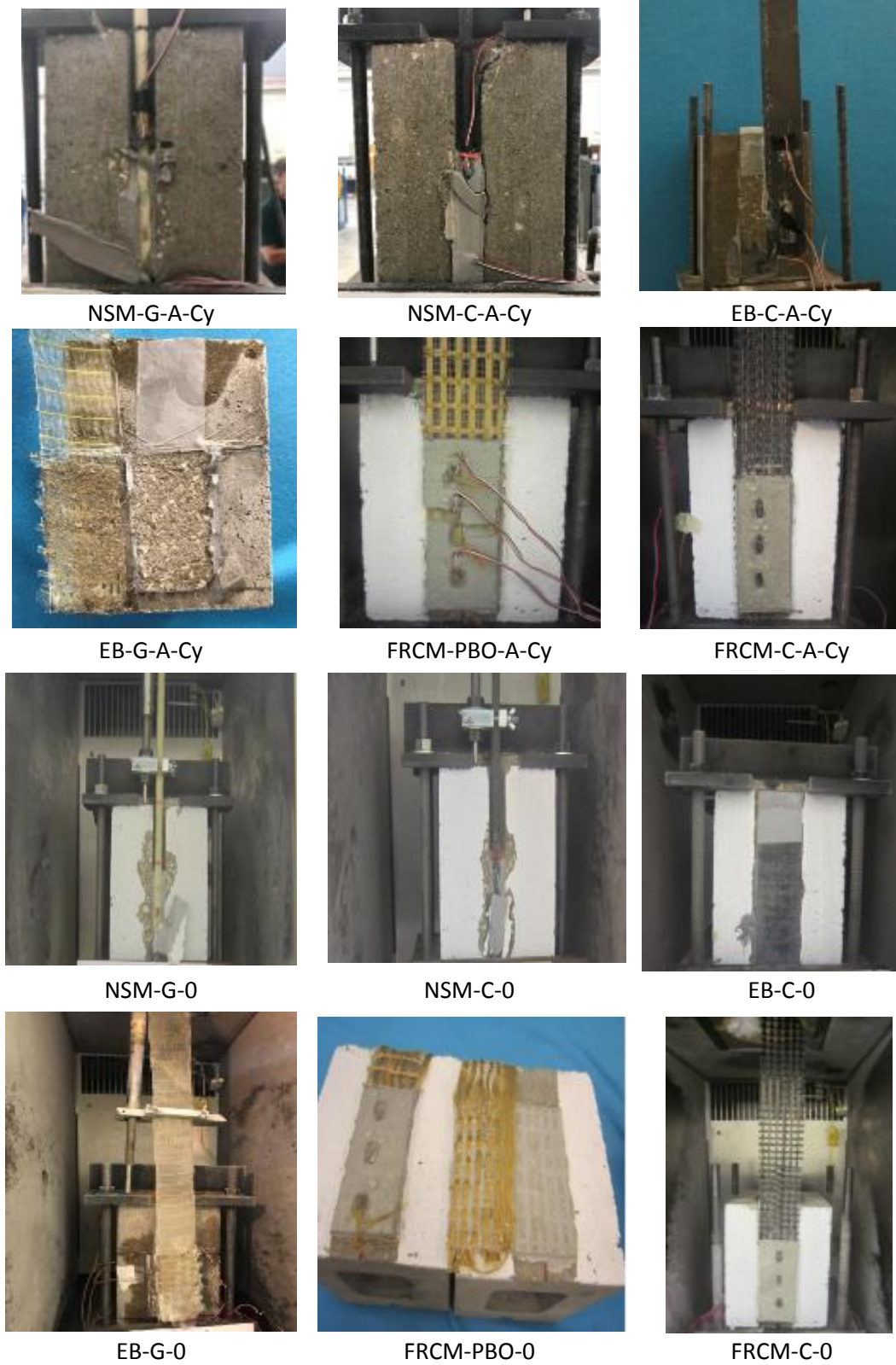
Figure10. Modes of failure for all strengthening system in different temperatures
