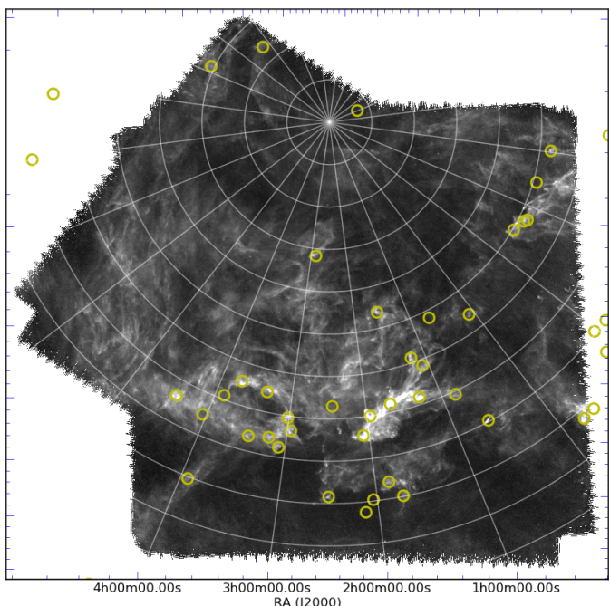
Fig. 16. The Polaris field observed by Planck ( top ) and Herschel ( bottom ) at 857 GHz ( 350 \mu\text{m} ). Structures that appear to be compact sources to Planck , shown with yellow circles, are revealed to be cirrus knots when observed at higher resolution. They are located in regions with bright backgrounds, which provides a proxy for identifying them. The declination grid has spacing of 30 arc-min.
