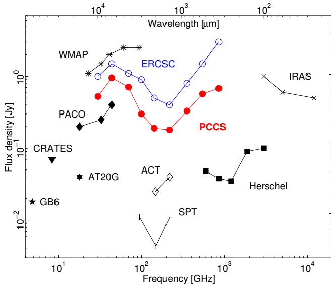
Fig. 18. The PCCS completeness level outside the Galactic plane (see Table 1) is shown relative to other wide area surveys. The ERCS completeness levels have been obtained from Planck Collaboration XIII (2011) up to 70 GHz and Planck Collaboration Int. VII (2013) for the other channels, while the WMAP ones are from González-Nuevo et al. (2008) up to 41 GHz and Lanz et al. (2013) for 61 and 94 GHz. The sensitivity levels for Herschel SPIRE and PACS instruments are from Clements et al. (2010) and Rigby et al. (2011), respectively. The other wide area surveys shown as a comparison are: GB6 (Gregory et al. 1996), CRATES (Healey et al. 2007), AT20G (Murphy et al. 2010), PACO (Bonavera et al. 2011), SPT (Mocanu et al. 2013), ACT (Marsden et al. 2014) and IRAS (Beichman et al. 1988).
