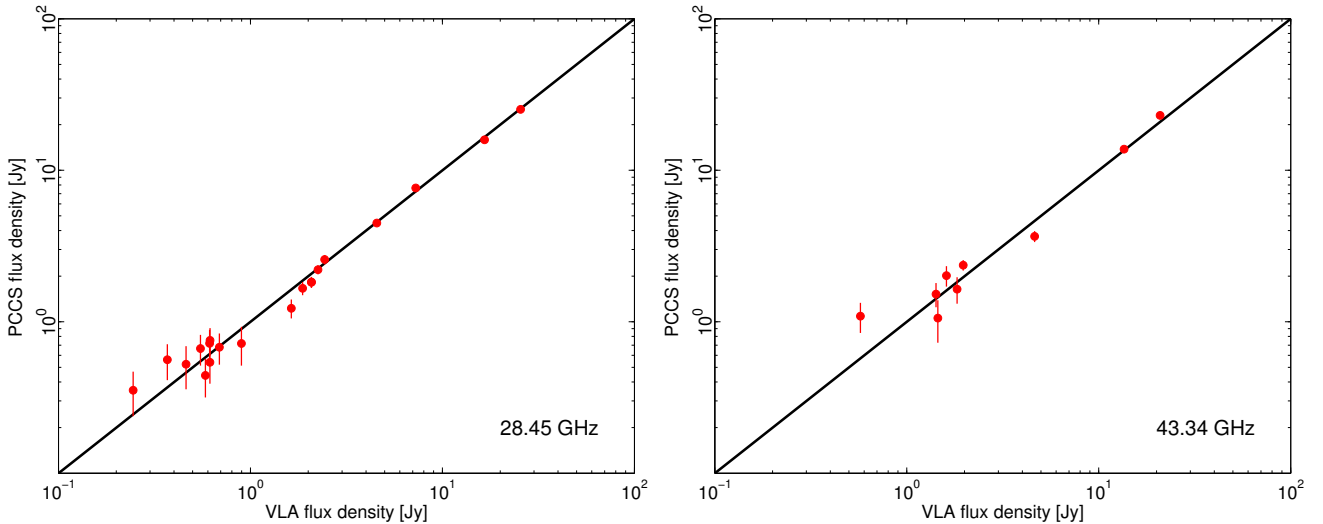
Fig. 11. Planck flux densities for bright sources observed within a month of VLA observations at that frequency. Planck values (APERFLUX) were colour-corrected and interpolated to \sim 28 GHz ( left ) and \sim 43 GHz ( right ).
