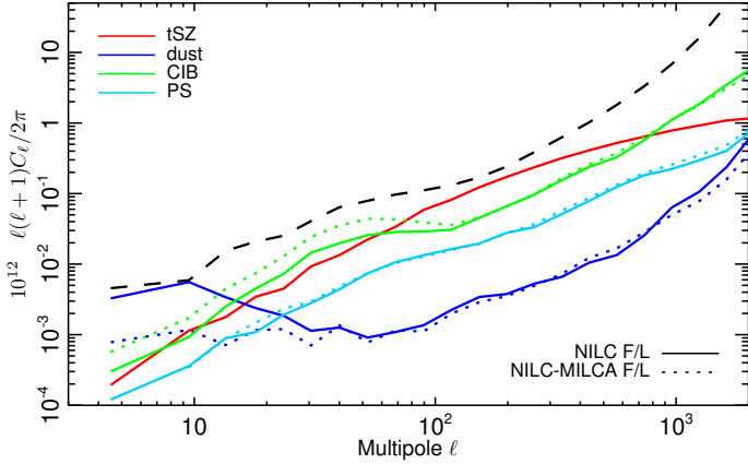
Fig. 4. Angular power spectrum of the main foreground contributions as estimated using the FFP6 simulations. We plot the diffuse Galactic emission (blue), clustered CIB (green) and point source (cyan) contributions, as well as the tSZ signal (red). The solid and dotted lines correspond to the NILC F/L and to the NILC-MILCA F/L cross-power spectra, respectively. For illustration we also show the Planck instrumental noise auto-power spectrum (dashed black line) in the MILCA Compton parameter map.
