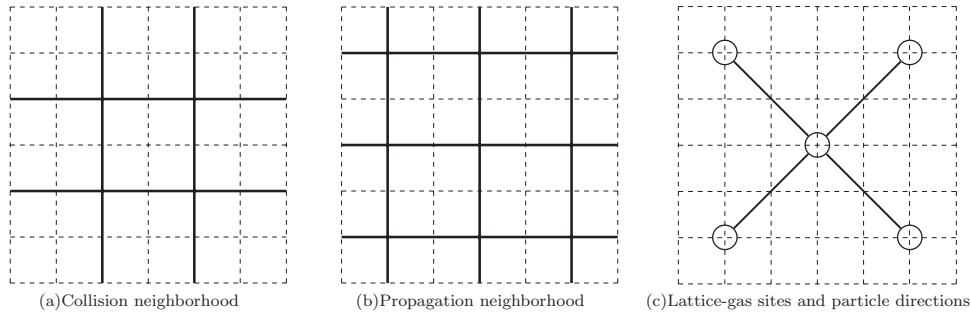
FIG. 3. Neighborhoods for collision (a) and propagation (b). The boundaries of the four cell blocks on which the rules shown in Figure 2 are applied are shown by the bold lines. Figure (a) shows the boundaries for the collision neighborhood. (b) The boundaries for the propagation neighborhood. (c) The correspondence between the cells of the partitioned automata and the lattice of the lattice-gas. Bold lines denote the directions along which lattice-gas particles move. Open circles denote sites of the lattice-gas.
