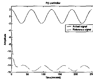
Fig. 3. Performance of a conventional controller without NNs.
