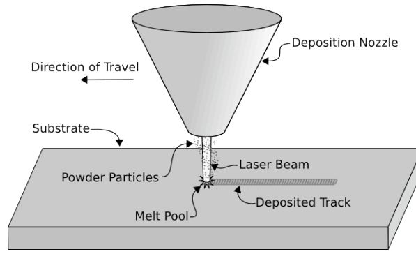
Fig. 1. Schematic of a typical laser deposition system
