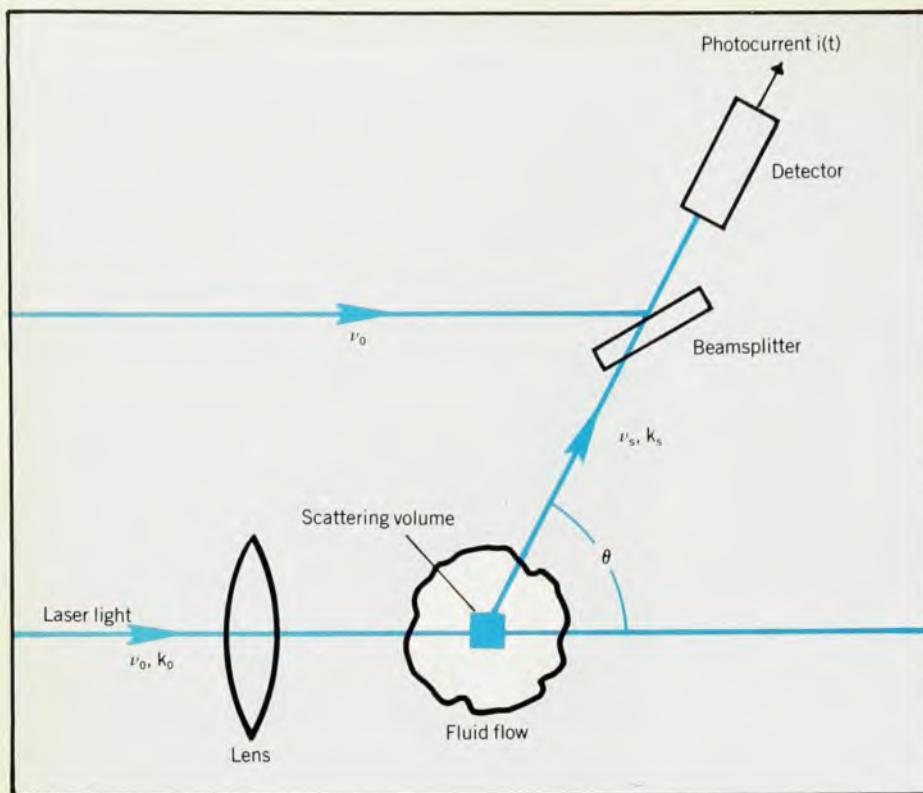
Laser Doppler system for velocity measurement. Laser light of frequency \nu_0 and wavevector \mathbf{k}_0 is focused on the fluid. The scattered light from a small volume, with its frequency Doppler shifted to \nu_s , passes through a beamsplitter and is mixed with the unshifted light. The alternating component of the photocurrent i(t) then oscillates at the Doppler frequency \nu_D = \nu_s - \nu_0 . Velocities of 10^{-4} – 10^5 cm/sec can be measured with this technique. Figure 3
