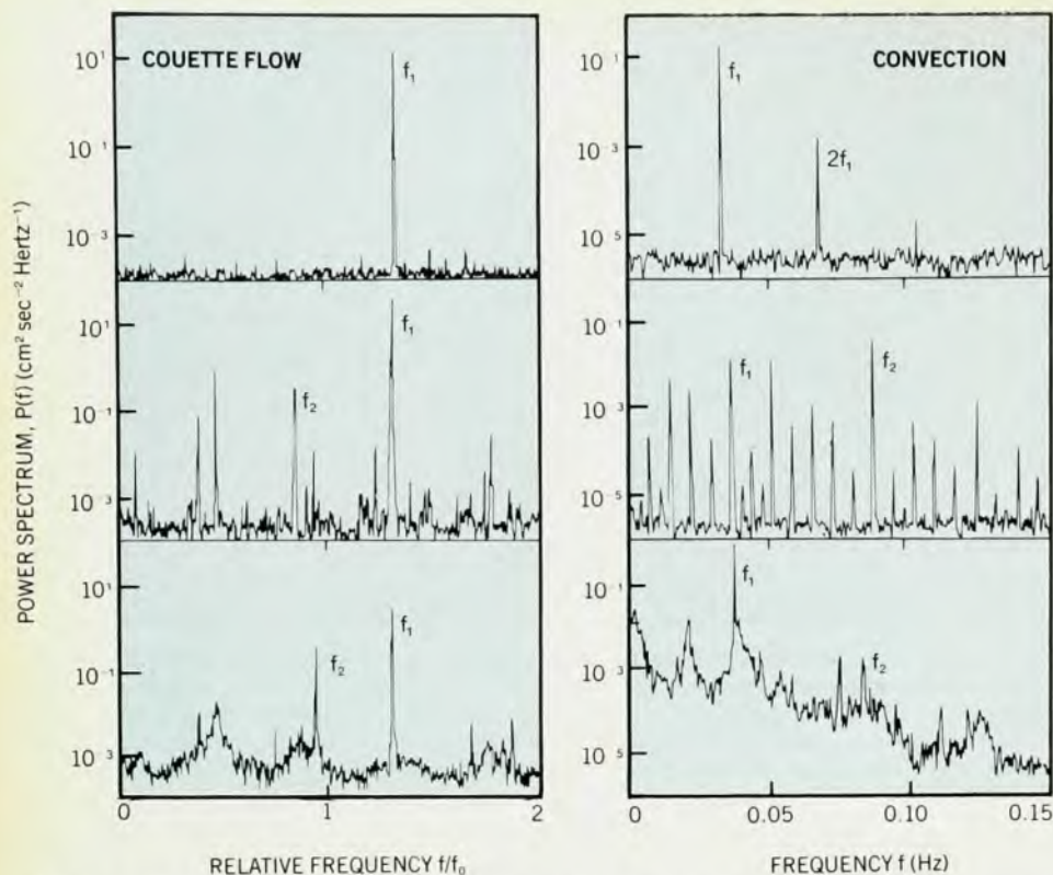
Power spectra of a component of the velocity of fluids in time-dependent Couette flow (left) and Rayleigh-Bernard convection (right). Different dynamical regimes are observed with increasing Reynolds number. The upper curves correspond to periodic flow, the middle ones to quasiperiodic flow with fundamental frequencies f_1 and f_2 , and the lower curves to chaotic flow containing both discrete frequencies and broad-band noise. In the data on the left, f_0 is the frequency of rotation of the inner cylinder of the Couette system (pictured in figures 2 a and b); the inner and outer radii are 22.2 and 25.4 mm, the height is 62.5 mm. The convection cell is rectangular, with a base 16 \times 28 mm and 8 mm in height. The Couette-flow spectra were obtained by R. Fenstermacher and the convection spectra by S. Benson. Figure 5
