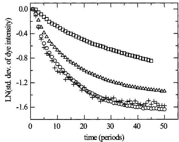
FIG. 4. Standard deviation of dye intensity as a function of time for p = 5 . ( \square ) Re = 25 ; ( \triangle ) Re = 55 ; ( \circ ) Re = 100 ; ( + ) Re = 170 . The decay rate of the variance grows with Re and saturates beyond Re \approx 100 .
