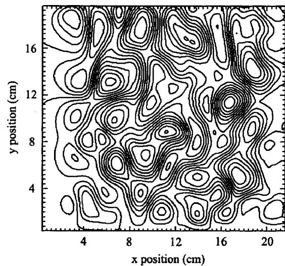
FIG. 2. Instantaneous stream function of the flow driven by the random magnet configuration at \text{Re} = 100 and p = 5 . The flow is instantaneously a random vortex array whose form is distorted with time, but that repeats periodically.
