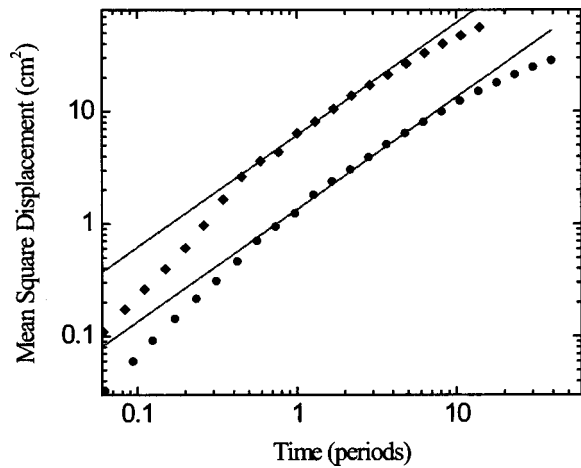
FIG. 9. Mean square displacement of particles for Re=100 , p=5 ( \blacklozenge ) and Re=100 , p=2 ( \bullet ). The solid lines show the linear (diffusive) scaling that best matches time range between 1 and 5 periods. These fits, along with Eq. (5), yield \Gamma_{\text{eff}}=3.1 \text{ cm}^2/\text{period} and 0.67 \text{ cm}^2/\text{period} , respectively.
