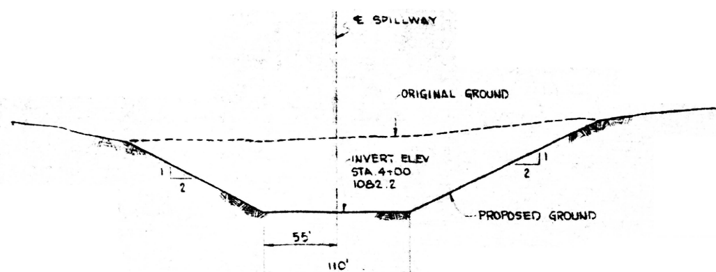
SECTION D-D LOOKING UPSTREAM SCALE 1" = 50'
