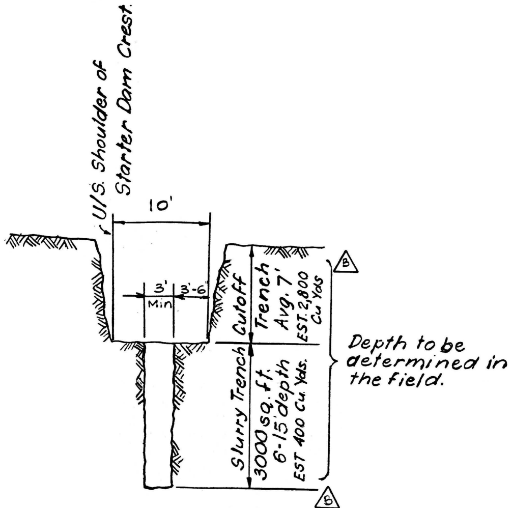
DETAIL 1 Scale: 1-in. = 10-ft
