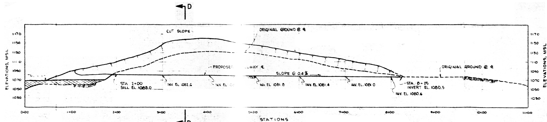
SECTION E-E (102) SPILLWAY PROFILE SCALE 1" = 50'
