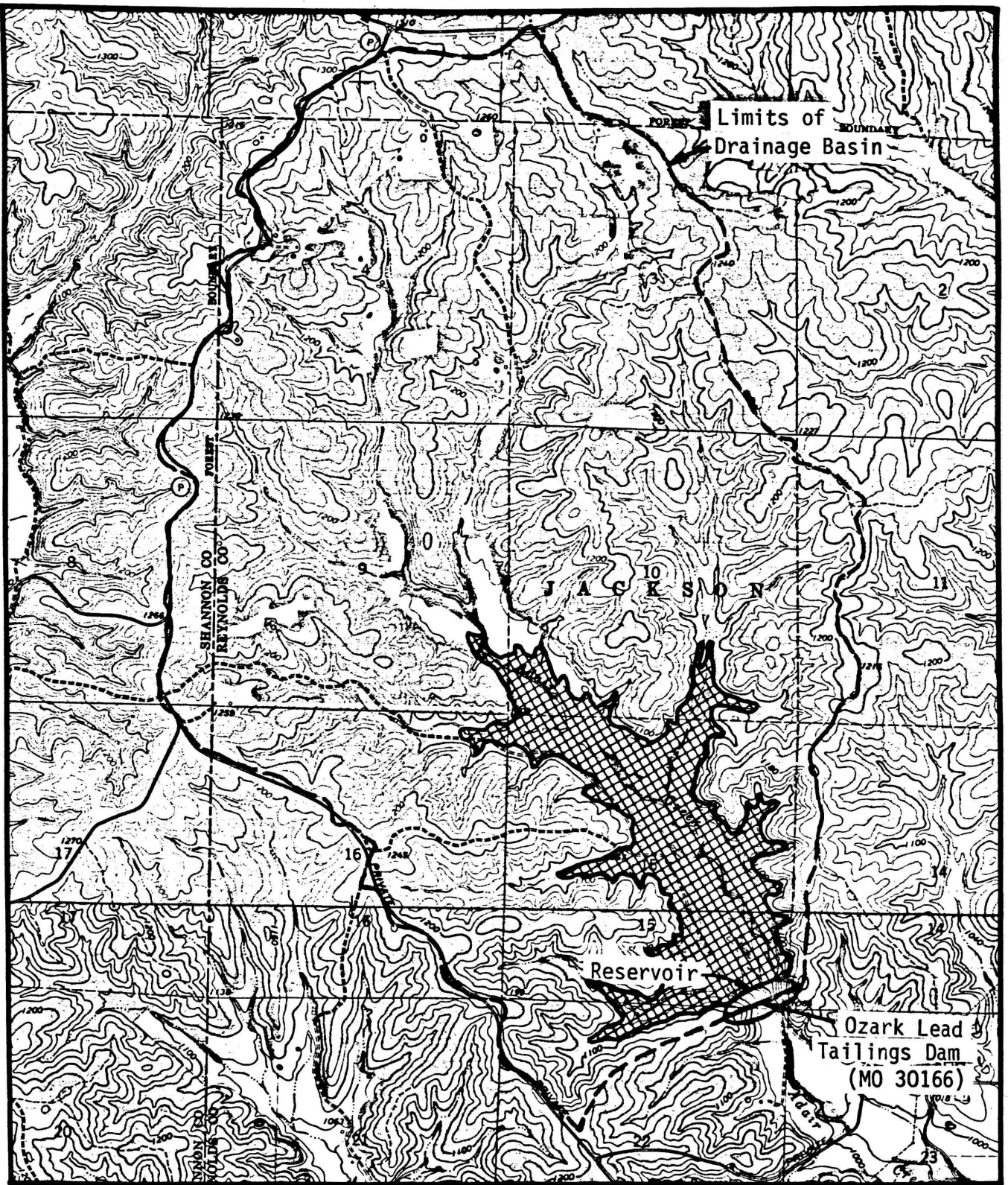
DRAINAGE BASIN AND SITE TOPOGRAPHY OZARK LEAD TAILINGS DAM MO. 30166 Fig. 2
