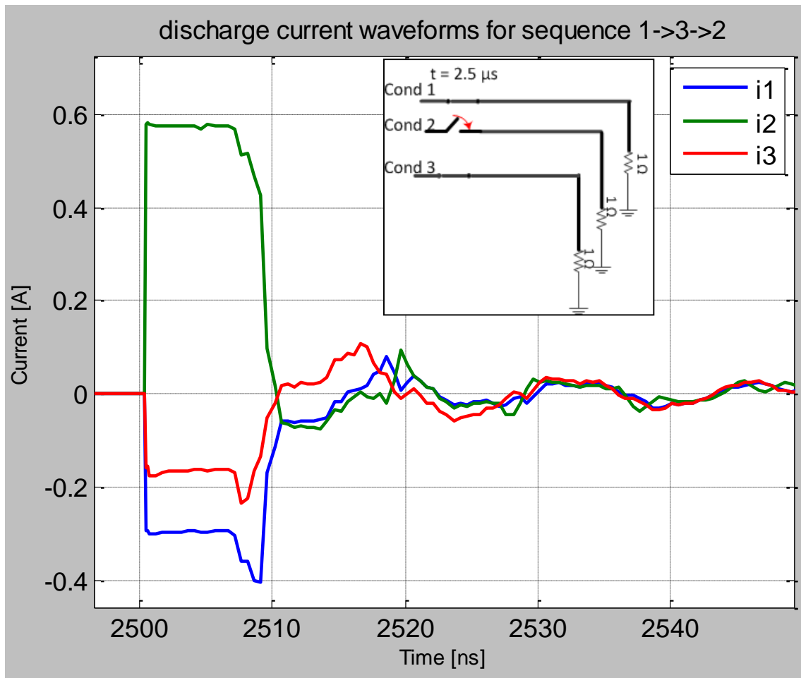
Figure 4.27. Discharge current on conductors 1 to 3 during the discharge of conductor 3 at 2.5us.
