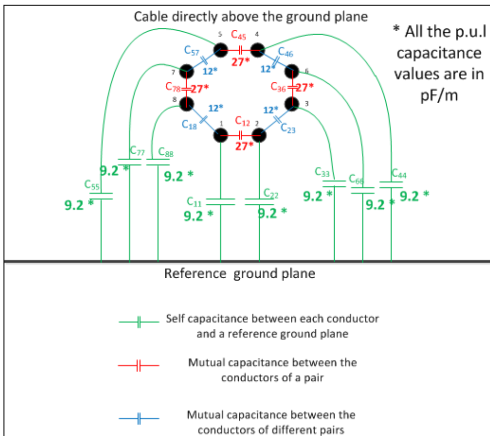
Figure 4.6. Equivalent capacitance model of a UTP cable placed directly above ground plane
