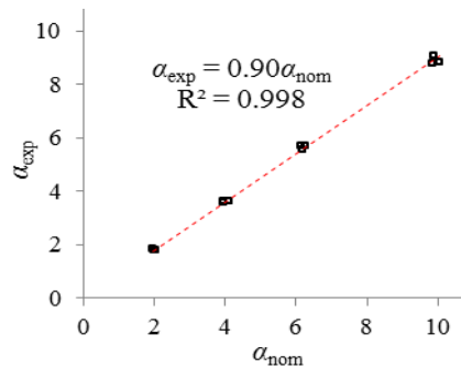
Figure 5.18. Comparison of experimental and nominal \alpha values
