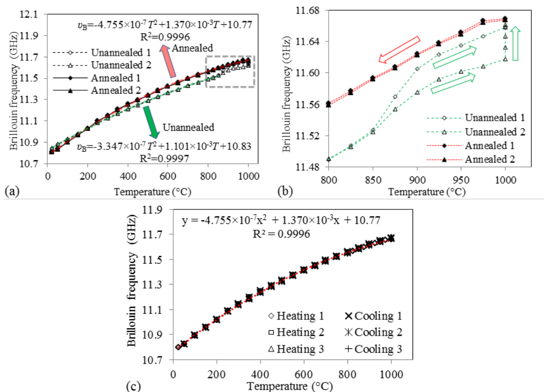
Figure 5.23. Brillouin frequency changes: (a) one cycle of 22\text{--}1000 \text{ }^\circ\text{C} before and after annealing; (b) one cycle of zoom-in 800\text{--}1000 \text{ }^\circ\text{C} before and after annealing; (c) three cycles of 22\text{--}1000 \text{ }^\circ\text{C} after annealing. The Brillouin frequency is denoted by \nu_B
