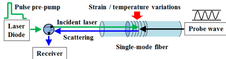
Figure 1.8. Illustration of PPP-BOTDA
