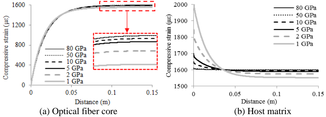
Figure 2.7. Longitudinal normal strain distributions
