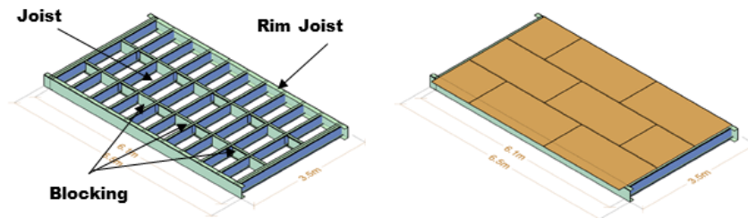
Figure 4 – Bare Frame and Frame with Sheathing : Test 13-FB4-M
