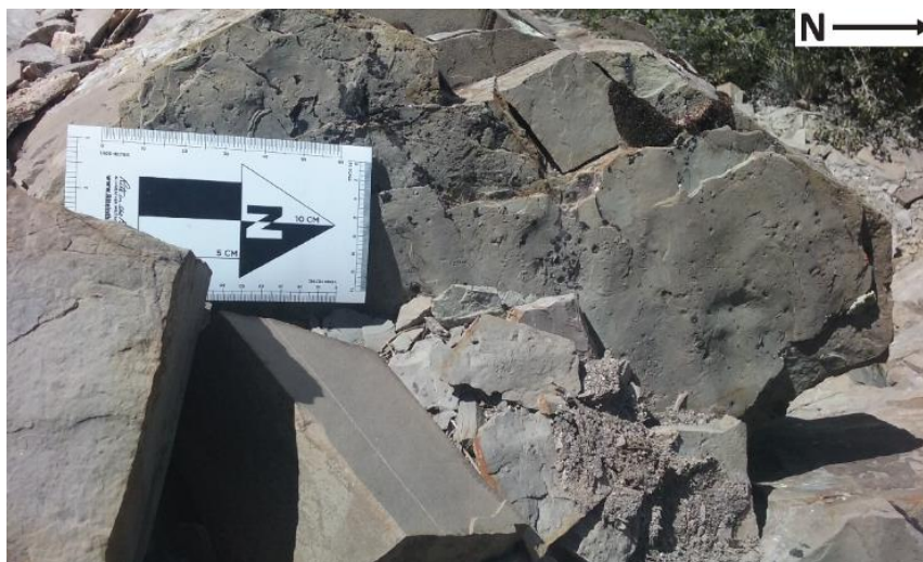
Figure D.6. Ripple marks on block of upright Triassic Virgin Limestone Member (TRmv). The crests show this is the upper surface of the bedding plane, which dips east (upright). However, the heavily disturbed nature of the top of the ridge suggests this piece may not be representative (not in place).
