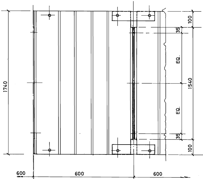
PLAN ON 'A-A'
