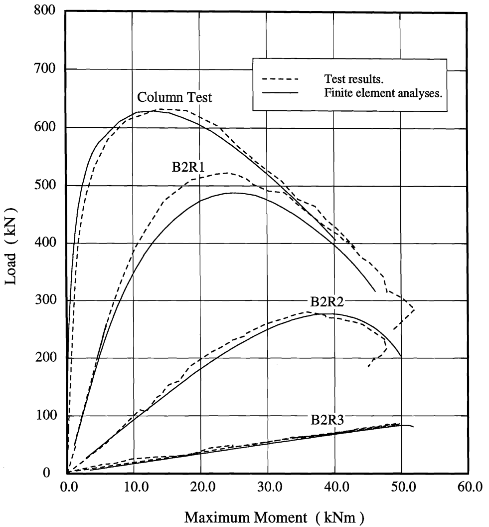
Figure 9: Maximum moment vs load for B2 series of interaction tests.
