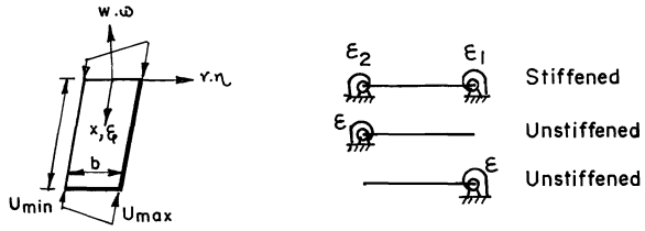
FIG.1 PLATE ELEMENT MODEL
