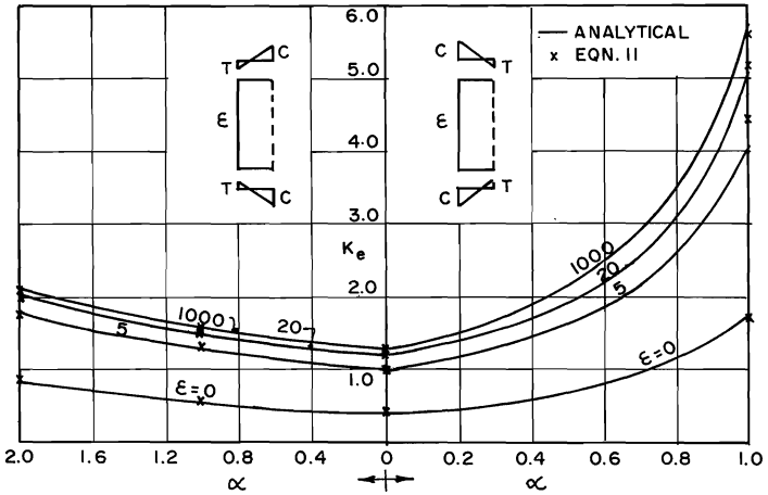
FIG.2 LOCAL BUCKLING COEFFICIENT OF UNSTIFFENED ELEMENTS
