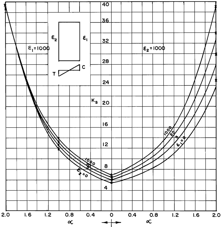
FIG.4 LOCAL BUCKLING COEFFICIENT OF STIFFENED ELEMENTS
