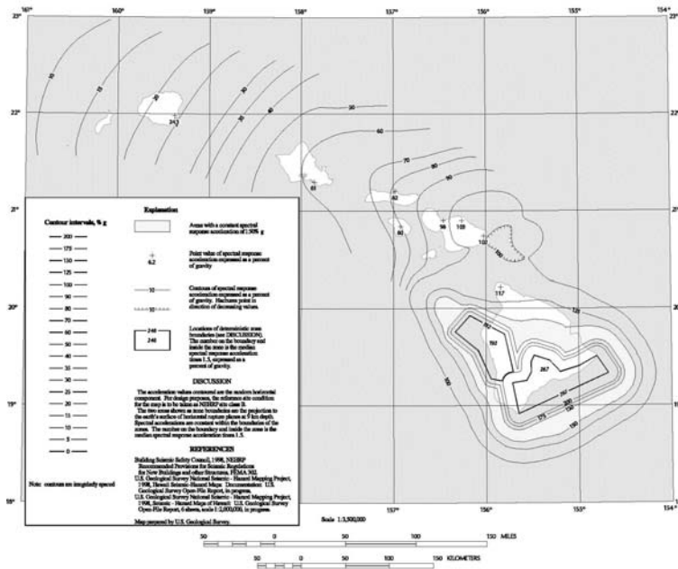
Figure 2.6.3-5 Maximum Considered Earthquake Ground Motion for Hawaii of 0.2 sec Spectral Response Acceleration (5% of Critical Damping), Site Class B
