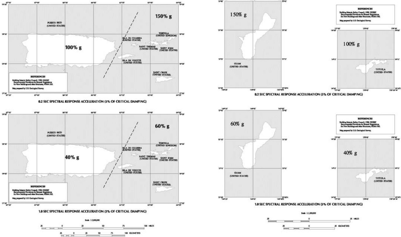
Figure 2.6.3-7 Maximum Considered Earthquake Ground Motion for Puerto Rico, Culebra, Vieques, St Thomas, St John, St Croix, Guam and Tutuilla of 0.2 and 1.0 sec Spectral Response Acceleration (5% of Critical Damping), Site Class B
