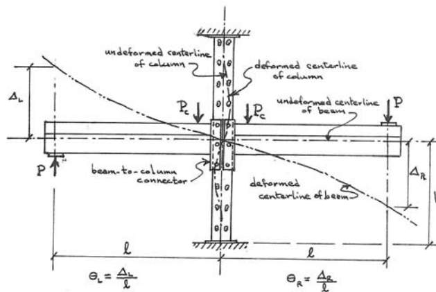
Figure 9.6.5-1 Test Set Up
