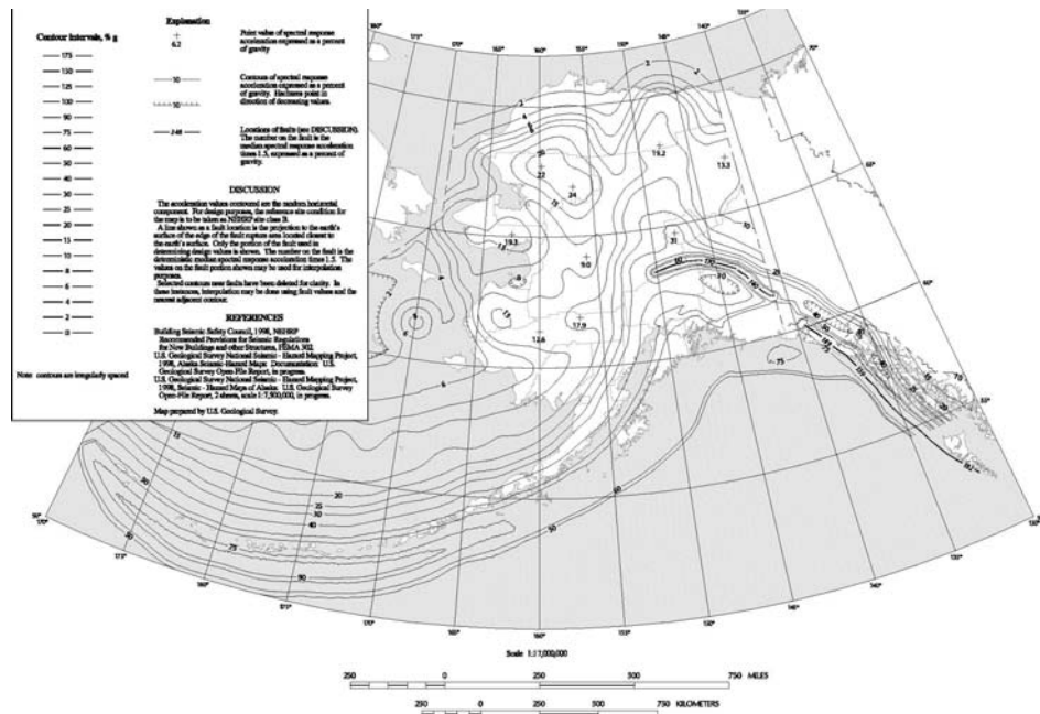
Figure 2.6.3-3 Maximum Considered Earthquake Ground Motion for Alaska of 0.2 sec Spectral Response Acceleration (5% of Critical Damping), Site Class B
