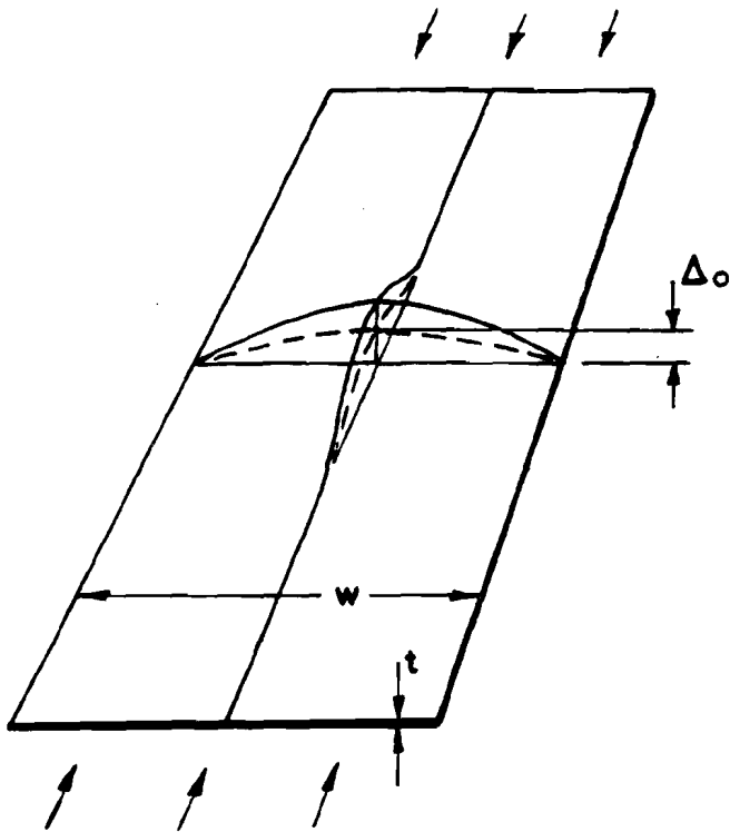
Fig. 1 Plate element in longitudinal compression. \Delta_o = initial out-of-flatness (ripple component).
