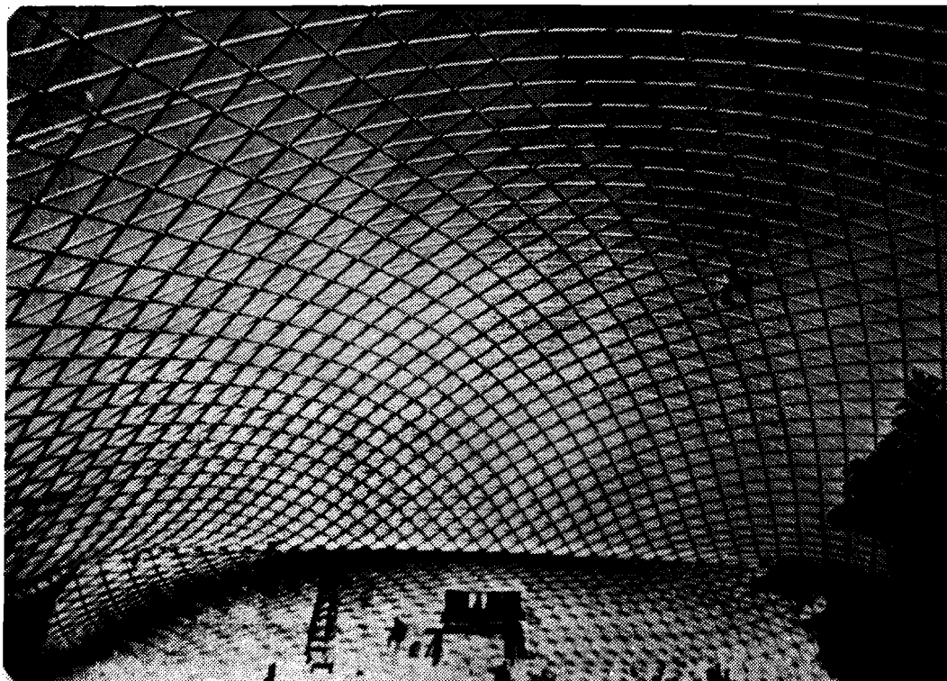
Fig. 2. Single layer space frame shell of arbitrary shape, Escuela Normal, Toluca, Mexico, 1966
