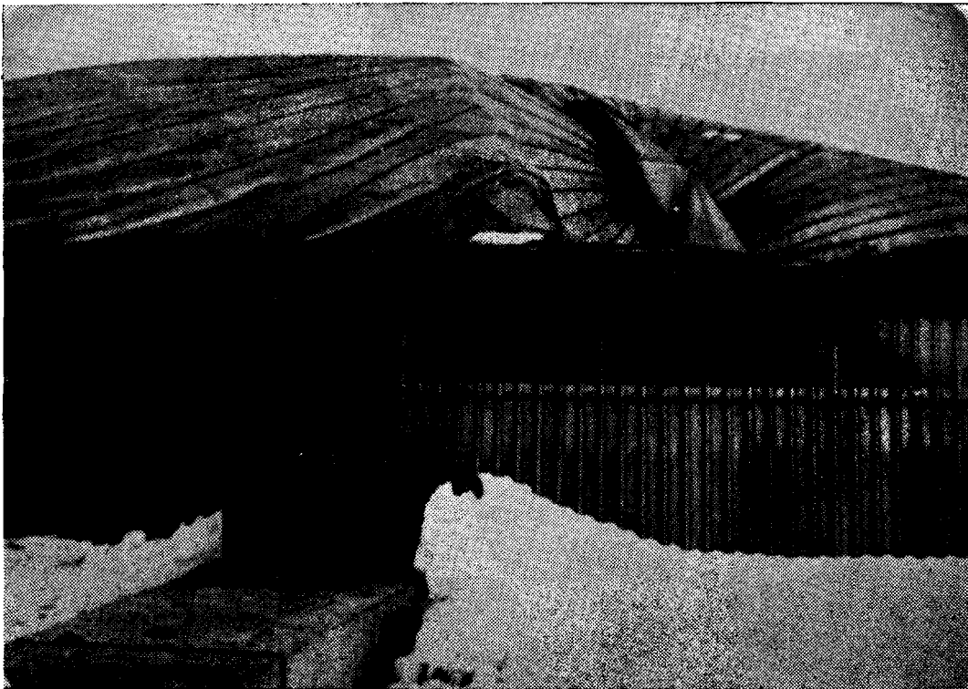
Fig. 10. View of water tank cover at Bradford, England, after failure under exceptional snow load
