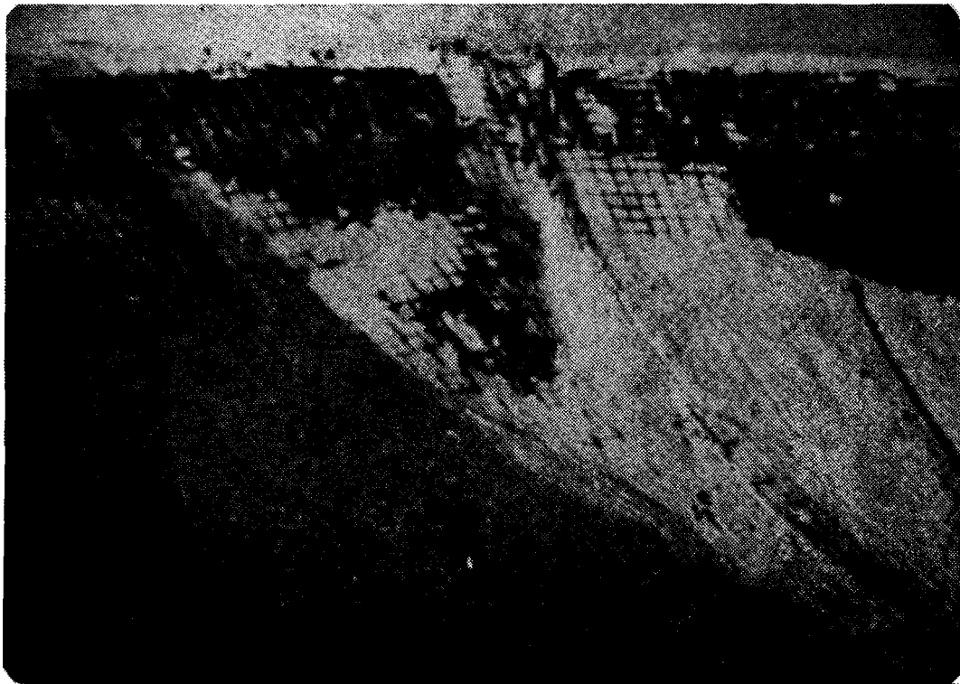
Fig. 6. View of the upper surface of Bucharest Dome after failure. Note part of cap at lower right corner
