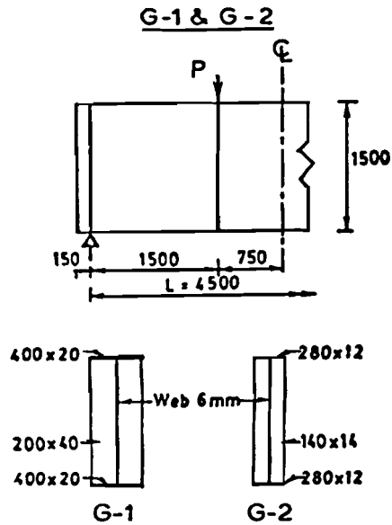
FIG. 1 DIMENSIONS OF GIRDERS
