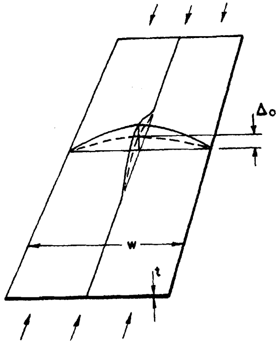
Fig. 1 Plate element in longitudinal compression. \Delta_0 = initial out-of-flatness (ripple component).
