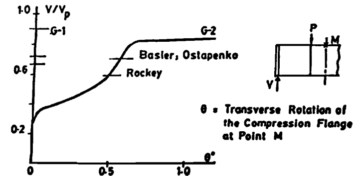
FIG. 4 TWIST OF THE COMPRESSION FLANGE
