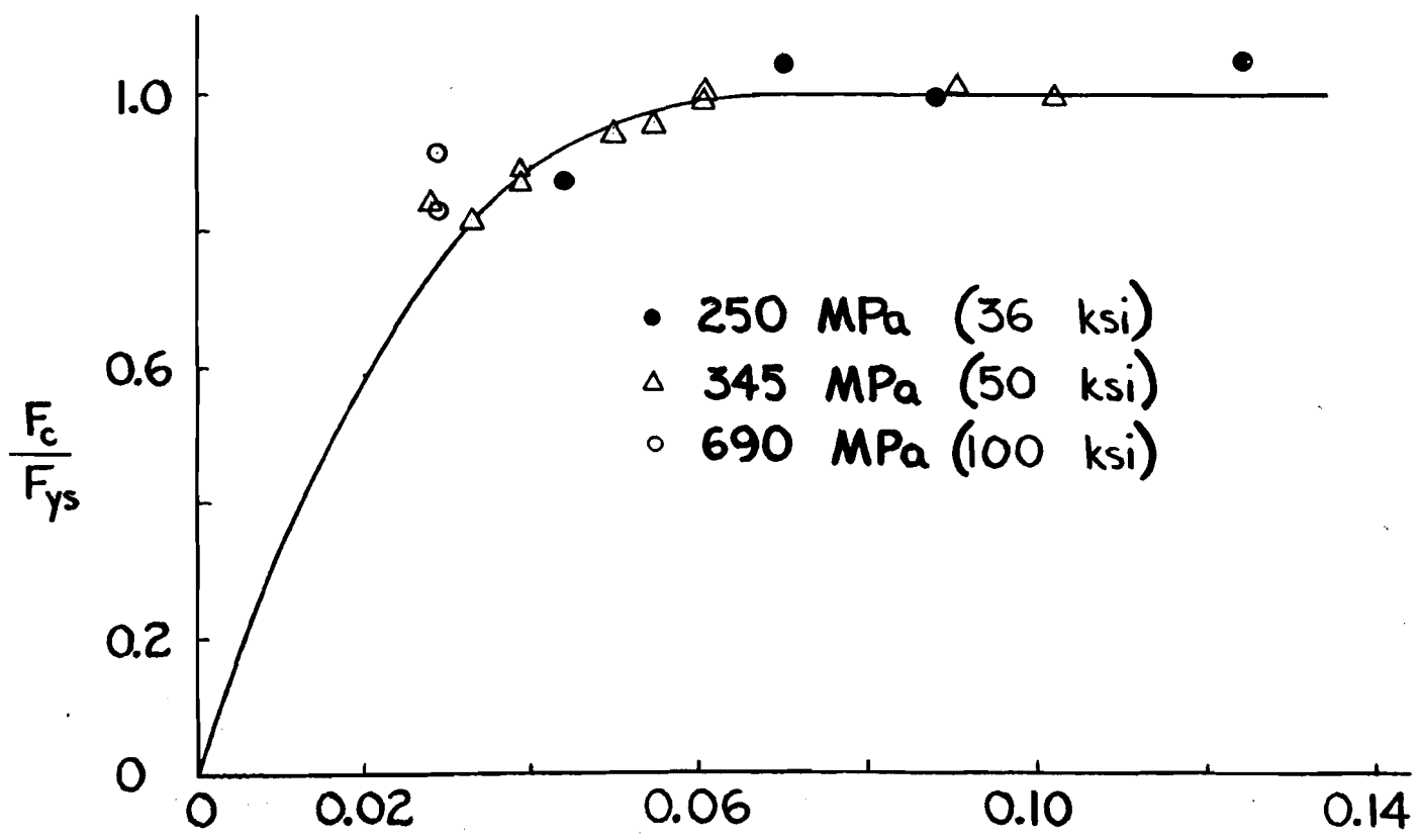
Figure 1 Typical Local Buckling Test
