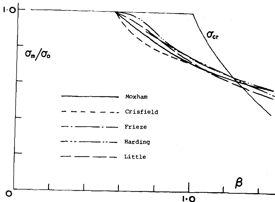
Fig. 4 Comparison of theoretical results for simply supported welded plates: c = 3t , moderate imperfection ( \Delta_0 = b/1000 ). Better consistency was obtained for non-welded plates.
