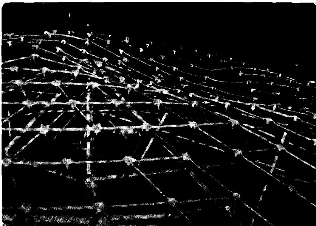
Fig. 8. View of experimental dome at University of Waterloo after test. Loading was by evacu-
