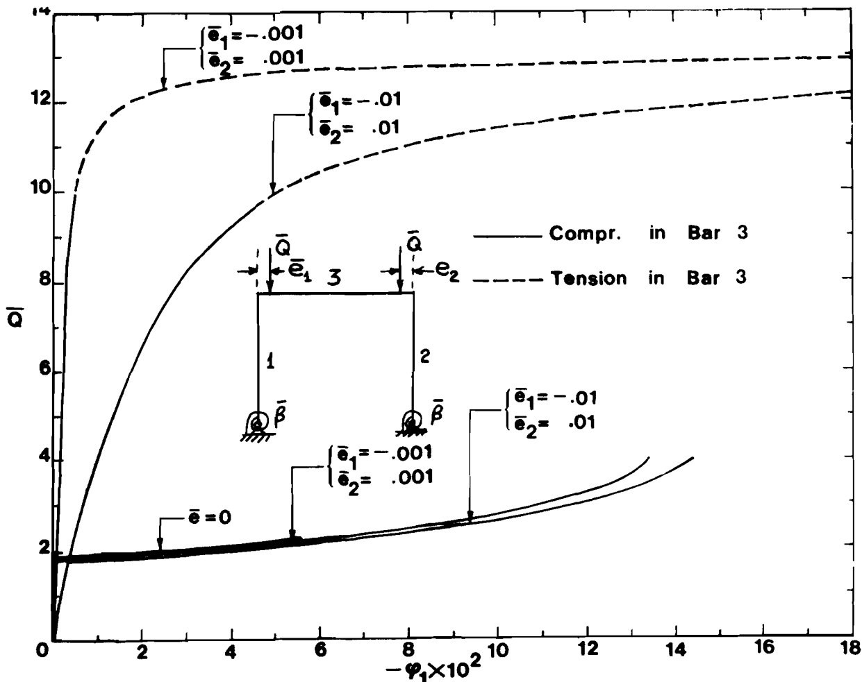
Figure 1. Equilibrium Response for a Symmetrically Loaded, Simply Supported Square Frame ( \lambda_k = 1,000 ; \bar{e} = 0 ; r_k = \mu_k = 1 ).
