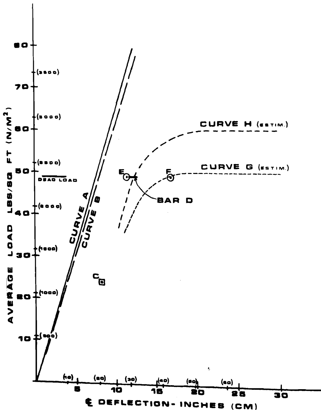
LOAD-DEFLECTION PLOTS
