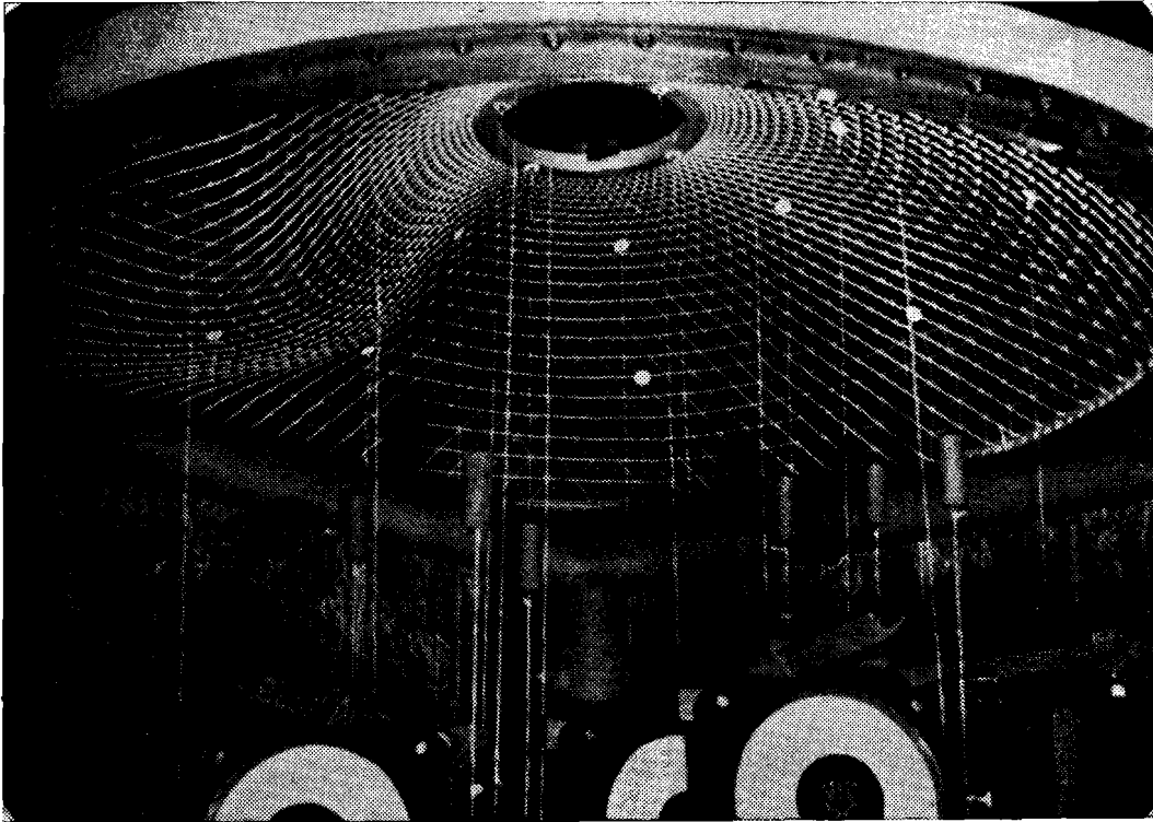
Fig. 9. View of experimental dome at University of Brno after test
