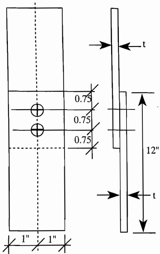
Figure 2. Connection Configuration for Two Screws in Shear.
