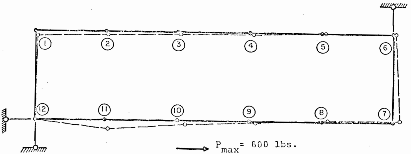
b) Displacements due to Load at node 10
