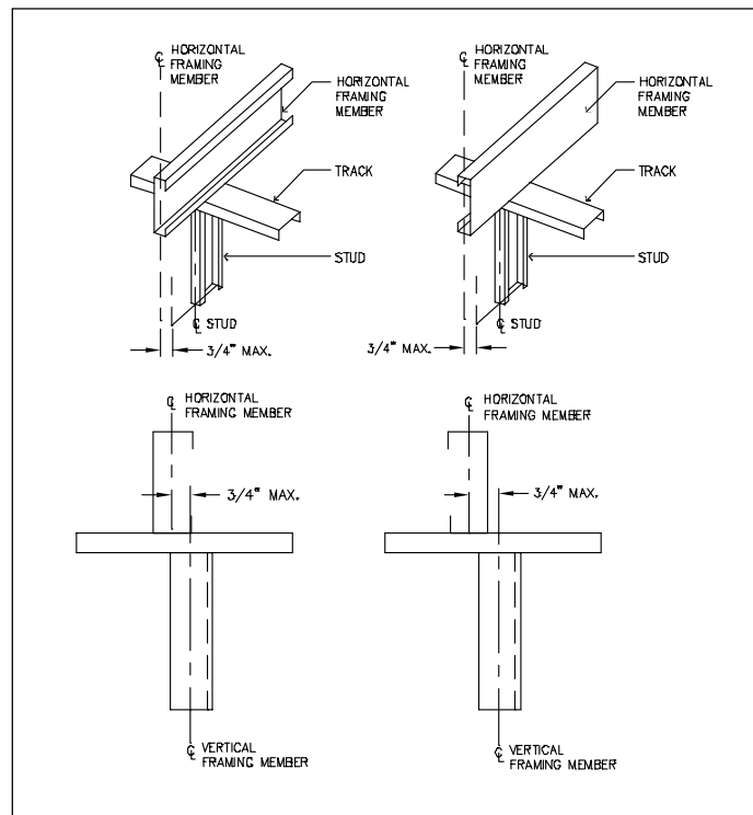
Figure C1-1 In-Line Framing
