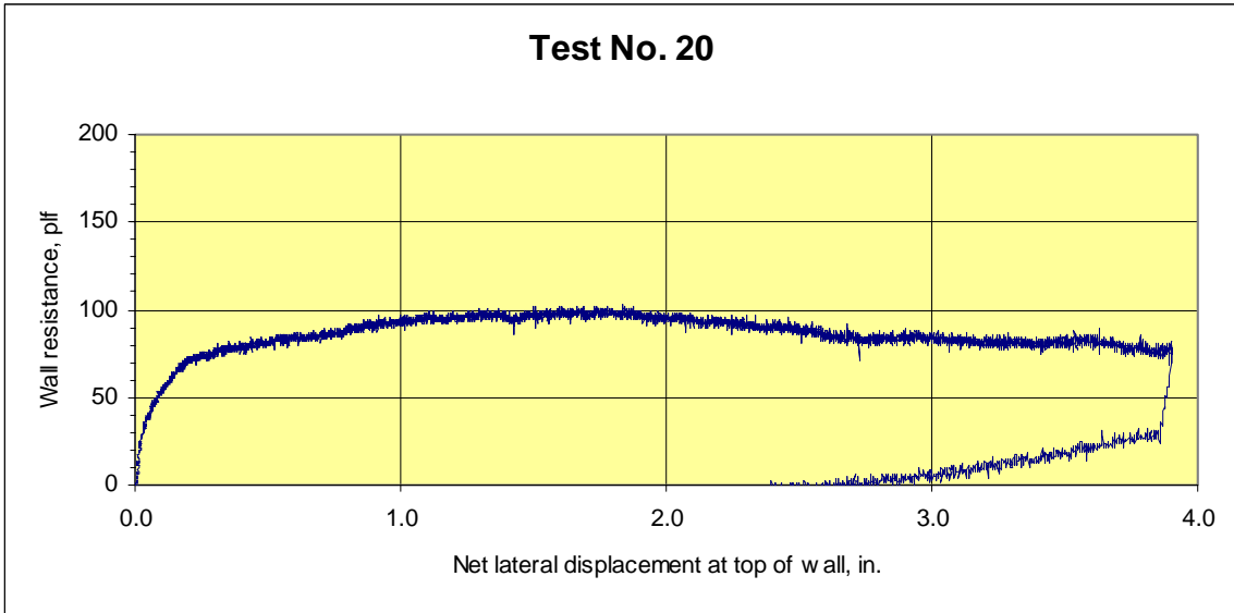
Figure A19. Response curve for Test 20
