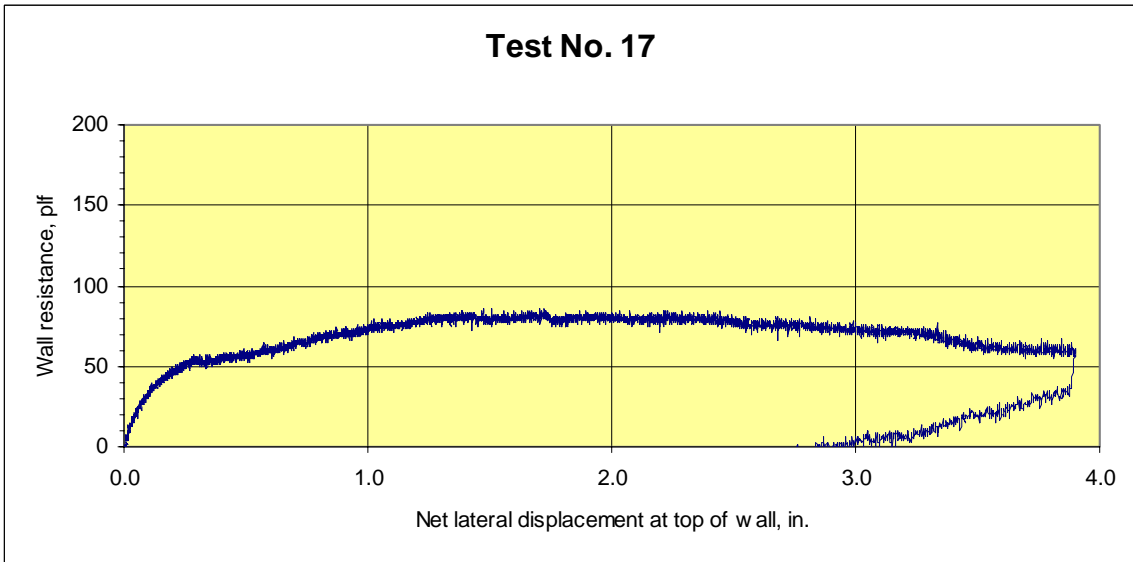
Figure A16. Response curve for Test 17
