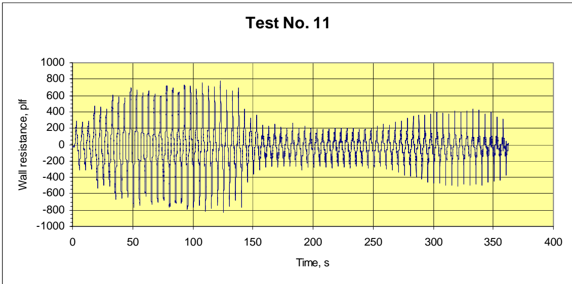
Figure B10. Resisting load history Test 11
