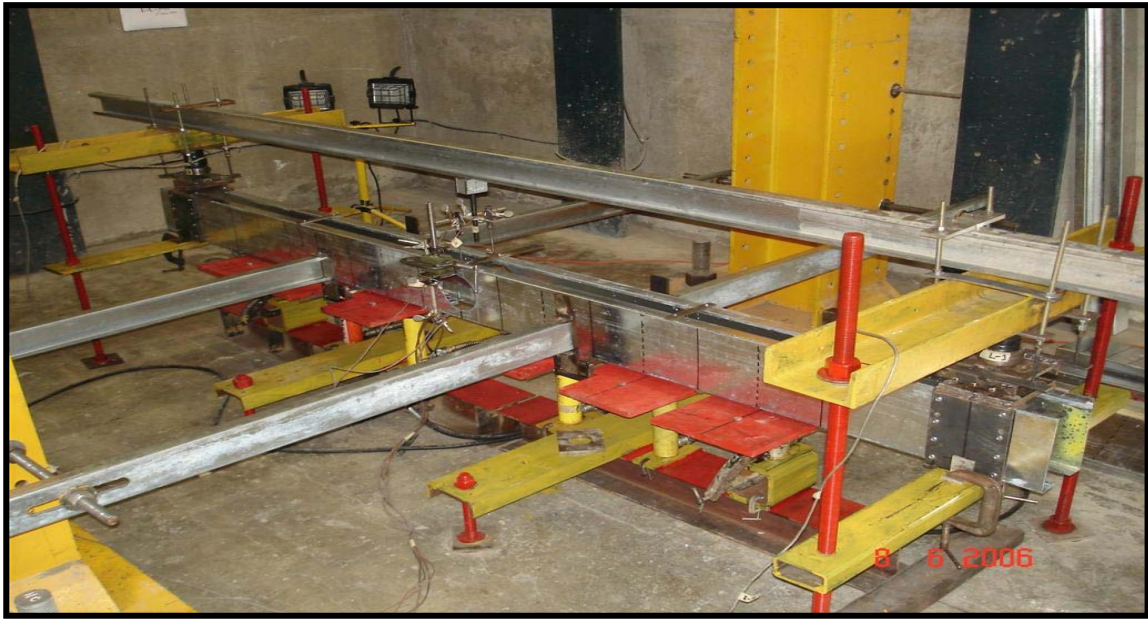
Figure 2.2 Photograph of the Flexural Test Setup
