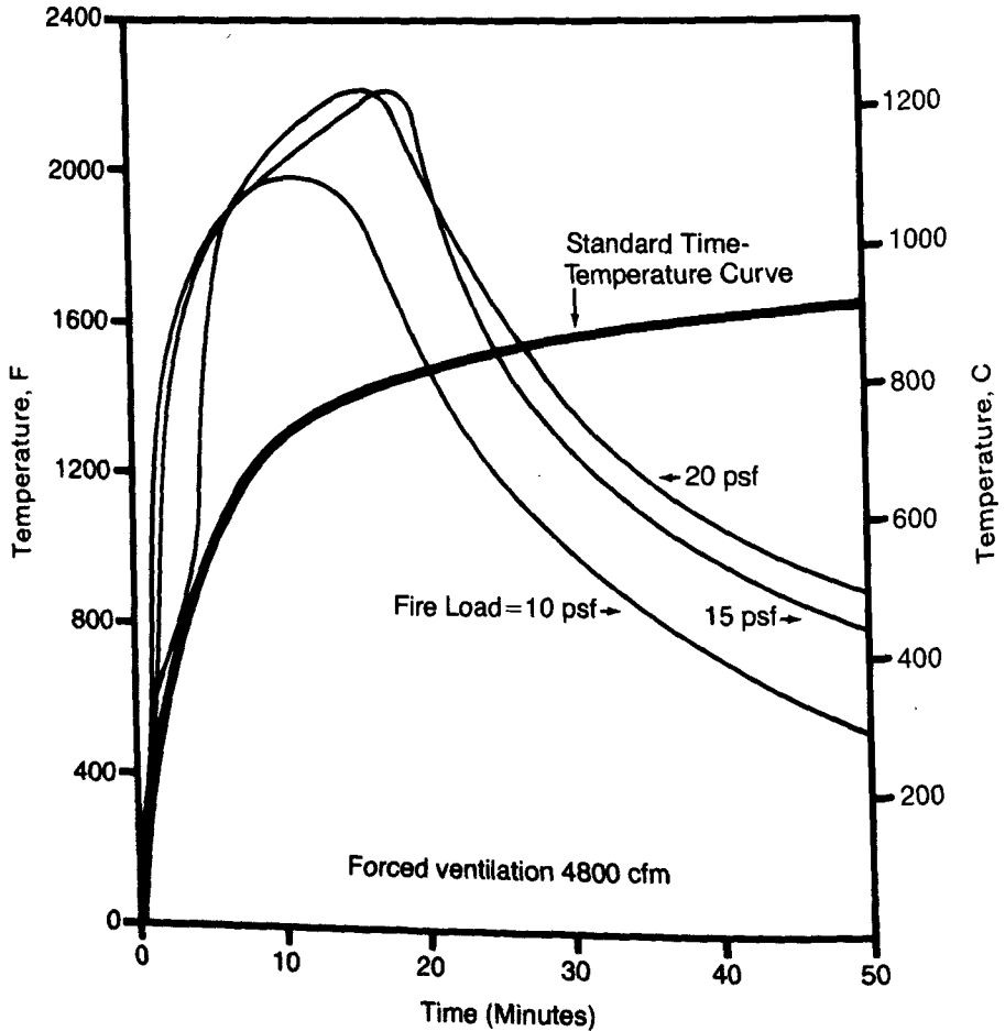
Figure 9. Effect of fire load on temperature recorded during burnout tests with forced ventilation.
