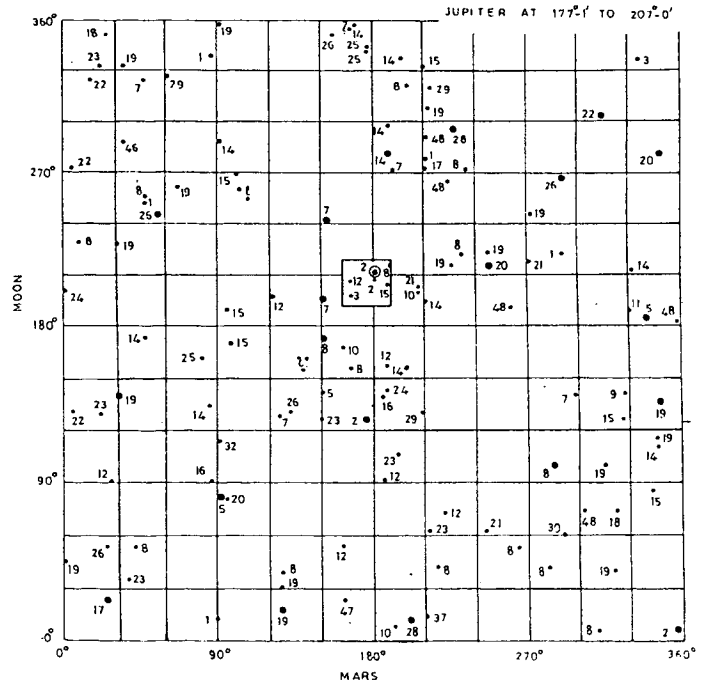
Fig. 2 Grid Showing Positions of Moon (Group-A), Mars (Group-B) Corresponding to Transit of Jupiter (Group-C) at 177^{\circ}-1' to 207^{\circ}-0' for Different Earthquakes
