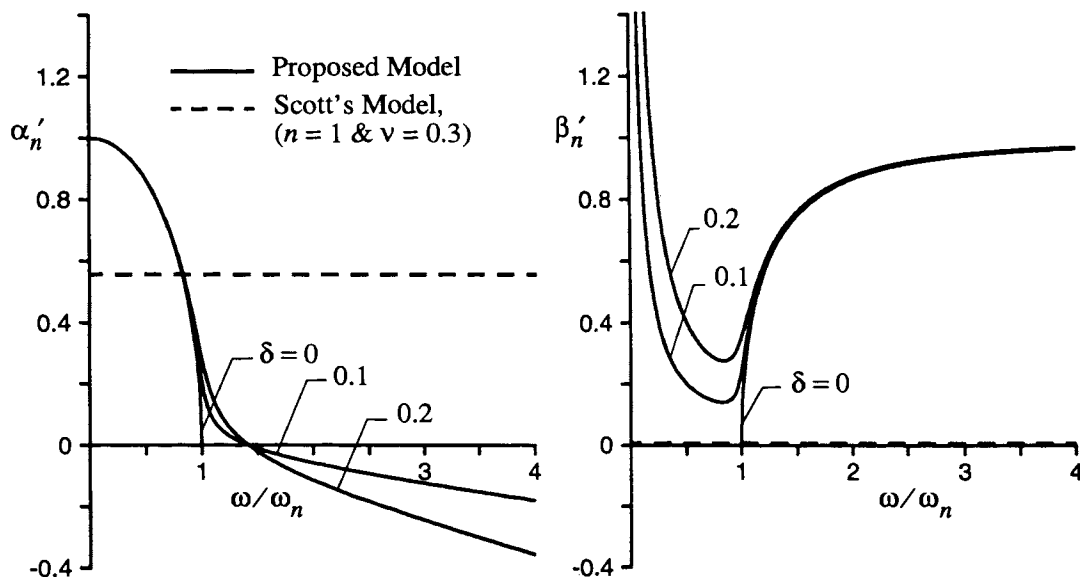
Fig. 17 Stiffness and damping factors for elastically constrained bar; straight wall.
