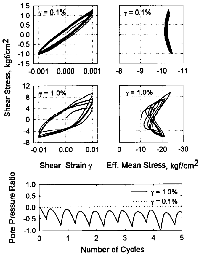
Fig. 5 Cyclic Responses for Dense Case
