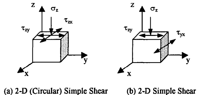
Fig. 4 Two-Directional Cyclic Loading
