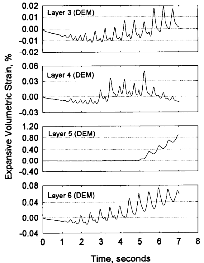
Fig. 9 Volume Change Responses for Dense Case
