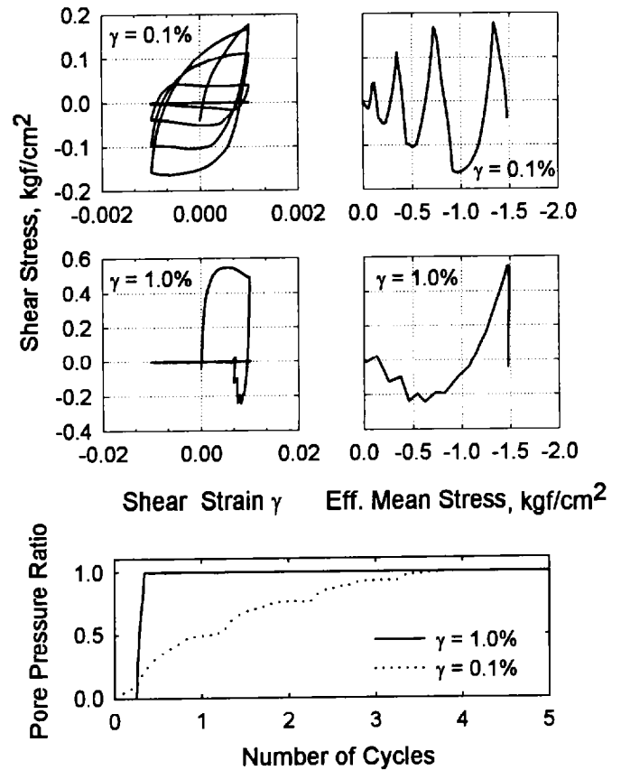
Fig. 6 Cyclic Responses for Loose Case
