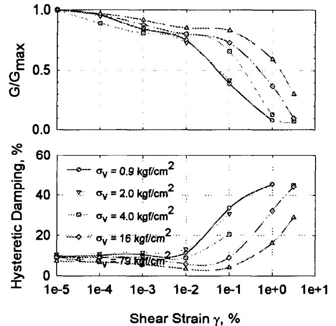
Fig. 3 Shear Modulus and Damping Curves
