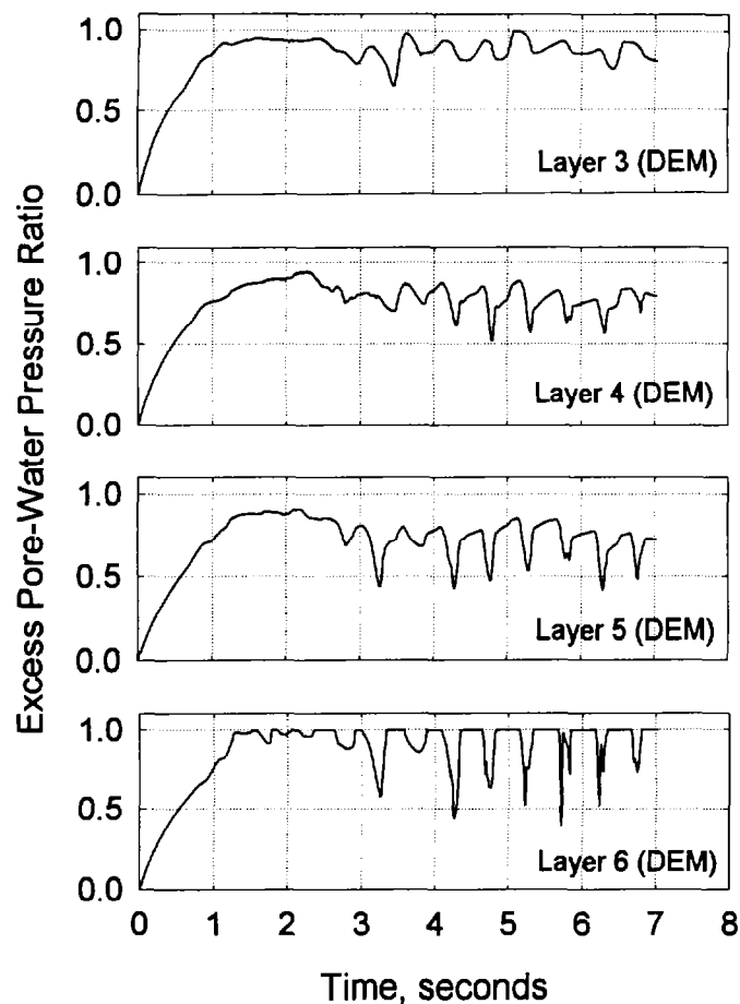
Fig. 11 Pore Pressure Responses for Loose Case
