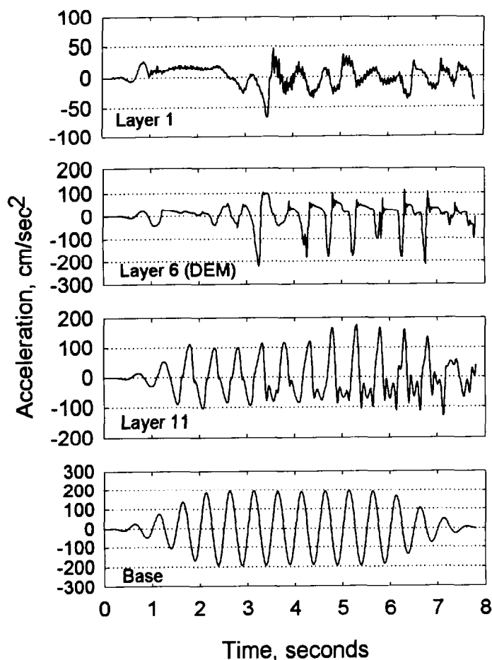
Fig. 10 Acceleration Responses for Loose Case
