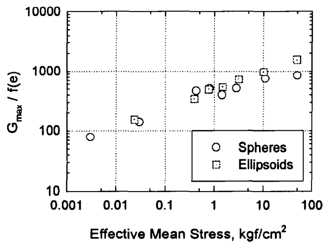
Fig. 2 Small-Strain Shear Moduli
