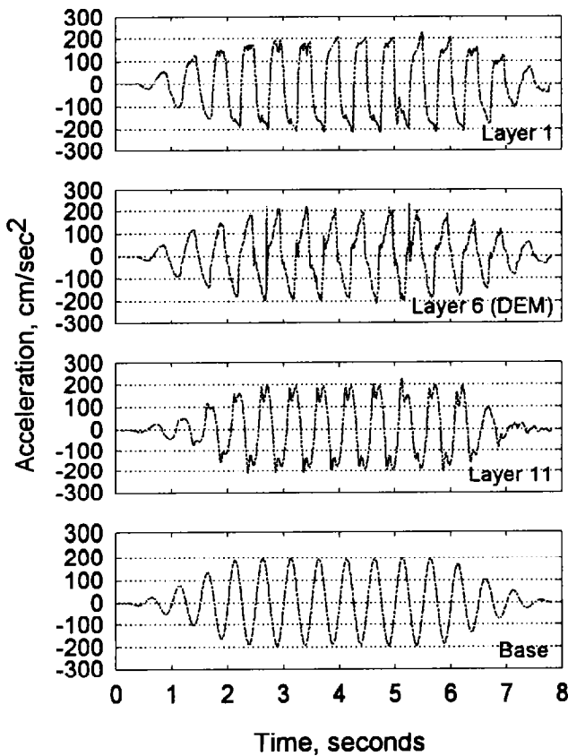
Fig. 8 Acceleration Responses for Dense Case
