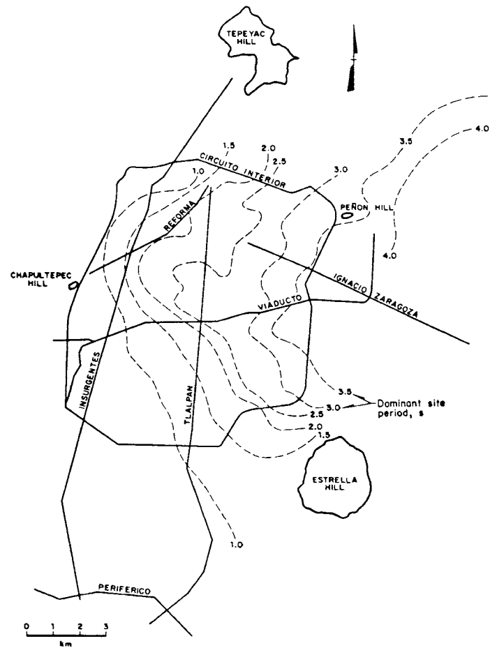
Fig 10. Dominant period contours in Mexico City (after Lermo et al, 1988)
