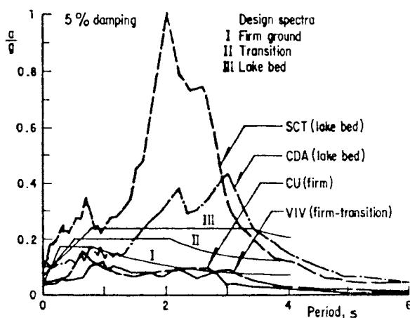
Fig 15. Normalized acceleration spectra for 5 % damping at several stations in the 1985 Mexico earthquake calculated from E-W components (after Meli and Avila, 1989)
