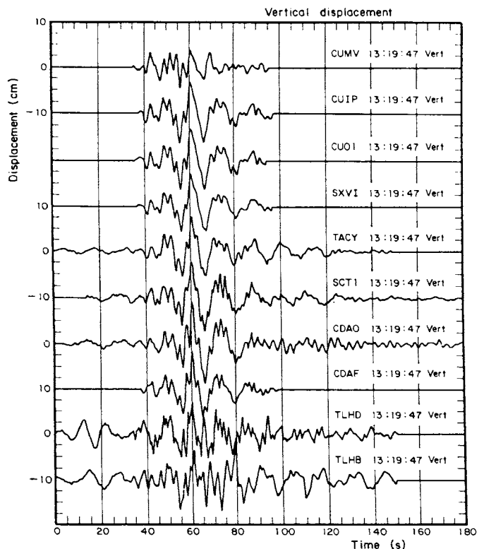
Fig 23. Vertical displacements in Mexico City during the September 19, 1985. For location of sites see fig 1 (after Campillo et al, 1986)
