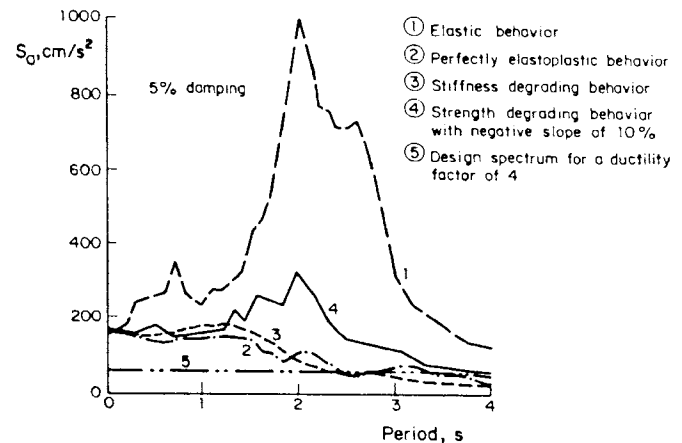
Fig 17. Inelastic acceleration spectra of the SCT-W record for a ductility factor of 4 (after Meli and Ávila, 1989)
