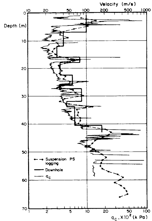
Fig 6. Shear wave velocity and cone penetration resistance. Virgin Texcoco Lake, zone III (after Jaime and Romo, 1988)
