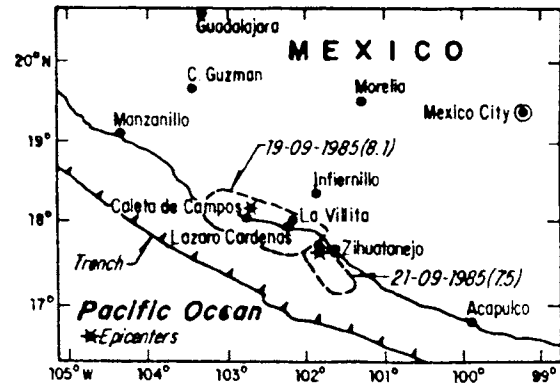
Fig 12. Epicenter for the September, 1985 earthquakes and areas of rupture in the subduction zone (after Meli and Ávila 1989)
