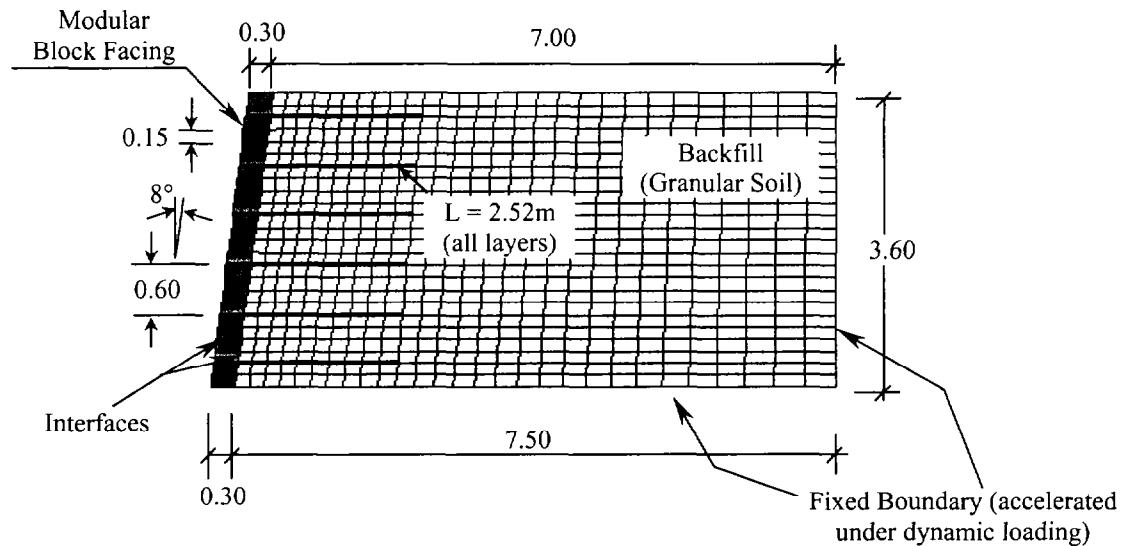
Fig. 1 Discretised model of segmental (modular block) retaining wall system at end of construction (dimensions are in metres).
