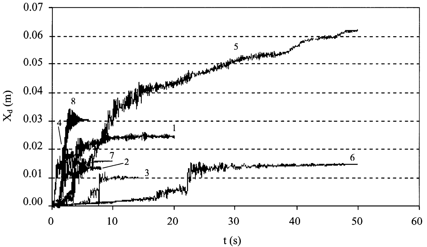
Fig. 4 History of facing lateral displacement at the top of wall subjected to input ground motions in Table 4 (all scaled to A=0.15g ).
