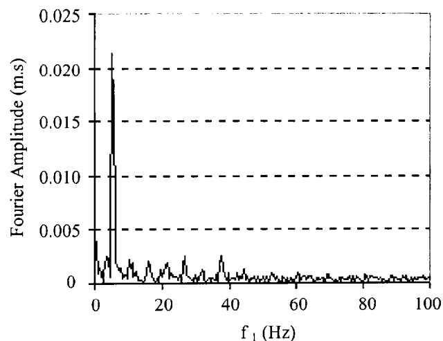
Fig. 2 Fundamental frequency of modular block retaining wall model from displacement response to sinusoidal impulse.
