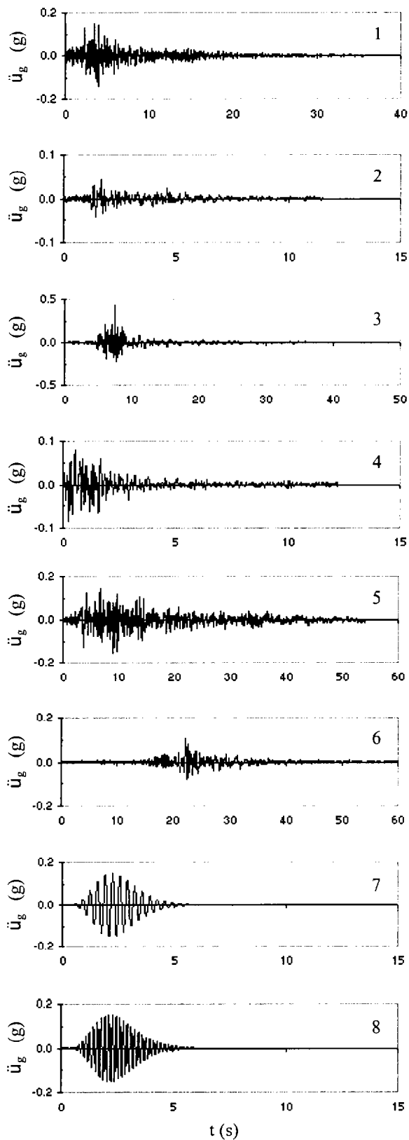
Fig. 3 Input acceleration histories applied to the modular block wall model (number in each figure refers to ground motion record in Table 4).
