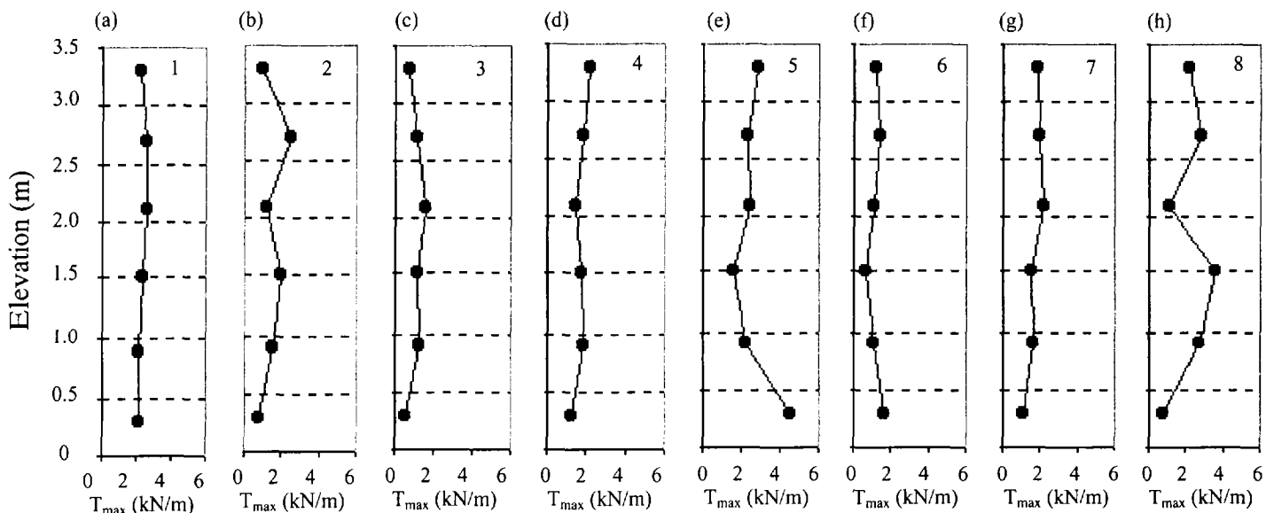
Fig. 5 Distribution of maximum reinforcement incremental load over the height of wall subjected to different input ground motions (number in each figure refers to ground motion record in Table 4).
