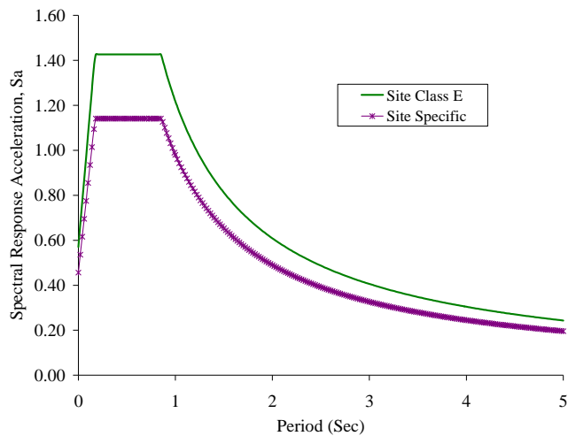
Fig. 3. Design Response Spectra for Existing Soil Conditions
