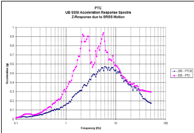
Fig. 27. PTCB SSSI Vertical Acceleration Response Spectra
