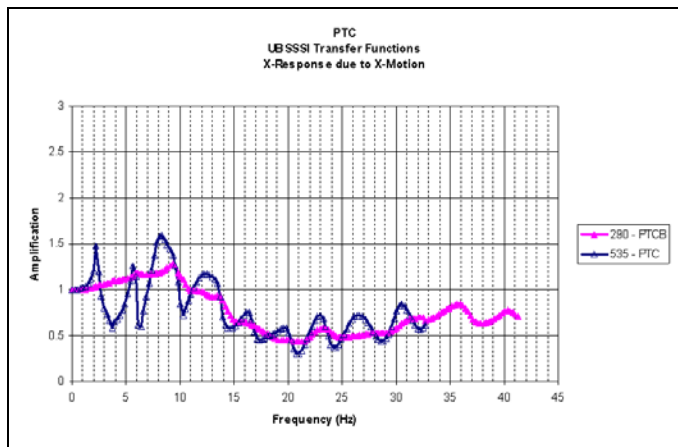
Fig. 18. PTCB SSSI EW Transfer Functions
