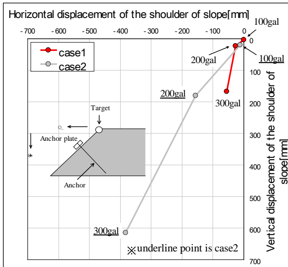
Fig. 13. The displacement of the shoulder of the slope of the model at each maximum acceleration amplitude for experimental cases 1 and 2.
