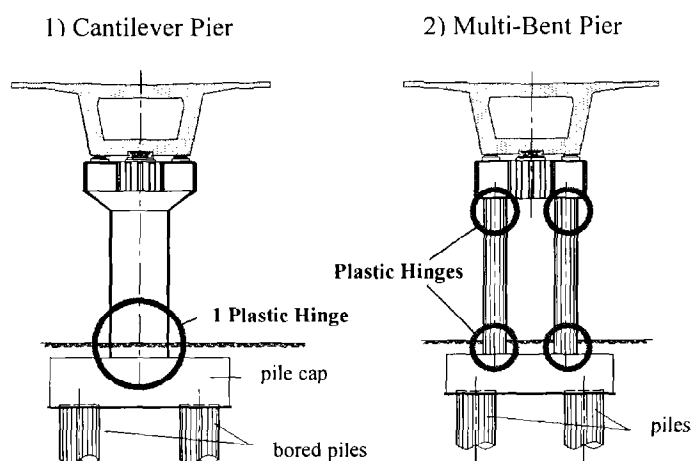
Fig. 2. Plastic hinges for different types of reinforced columns
