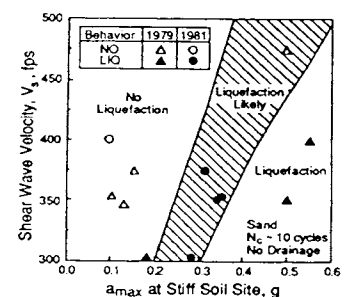
Comparison of Field Performance and Predicted Behavior in Imperial Valley, California
