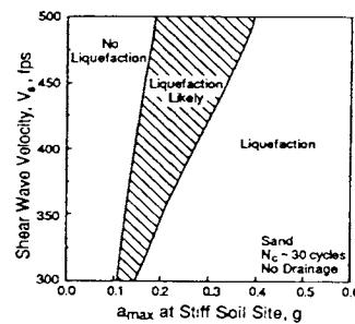
Liquefaction Potential Chart Based on V_s of Sand Layer and 30 Cycles of Strong Motion
