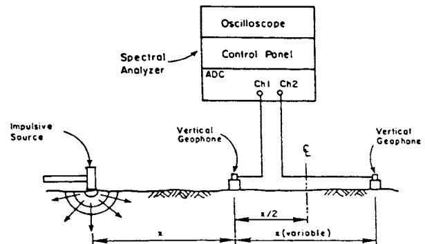
(a) General Configuration of SASW Tests
