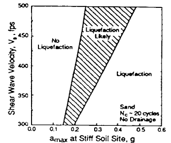
Liquefaction Potential Chart Based on V_s of Sand Layer and 20 Cycles of Strong Motion
