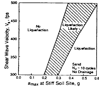
Liquefaction Potential Chart Based on V_s of Sand Layer and 10 Cycles of Strong Motion
