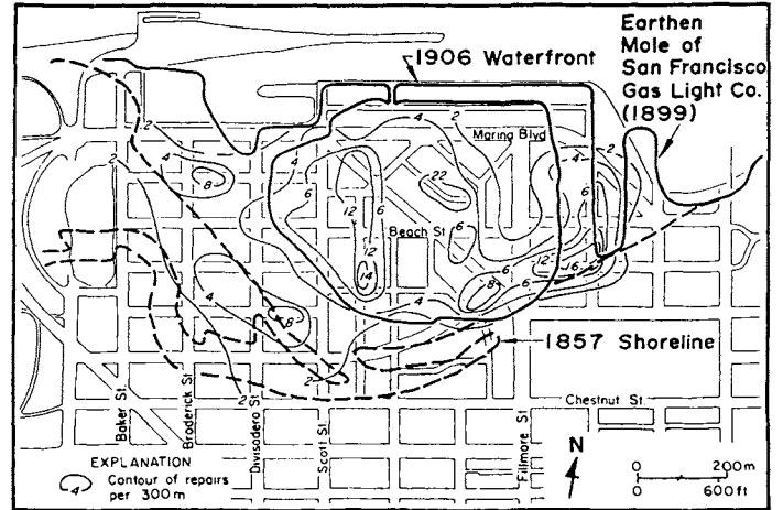
Figure 6. Repairs to MWSS Mains, Service Lines, and Sections Near Gate Valves in the Marina District
