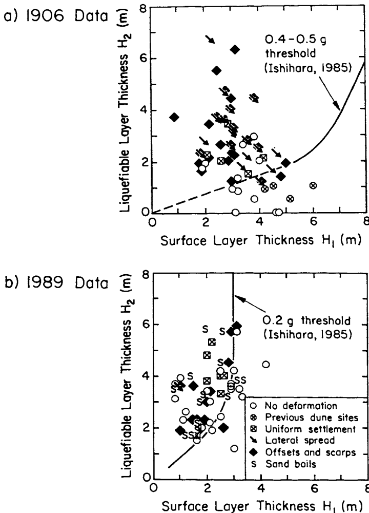
Figure 26. Ground Deformation in the South of Market and Mission District Plotted with Respect to Subsurface Geometry for the 1906 and 1989 earthquakes
