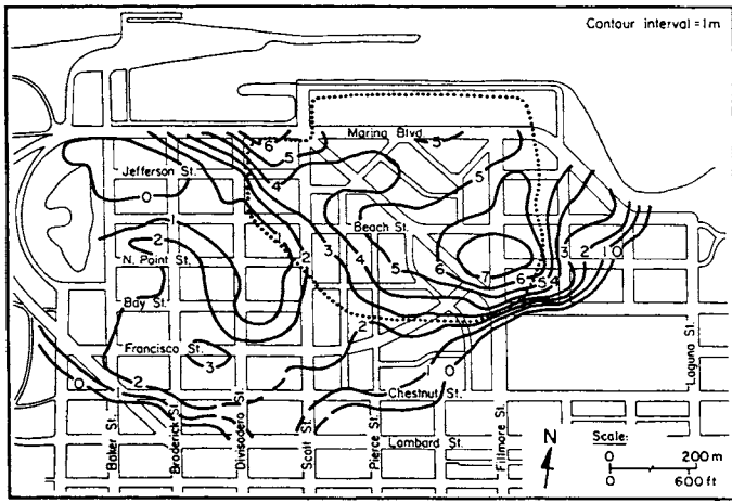
Figure 4. Thickness of Submerged Fill Deposits in the Marina District
