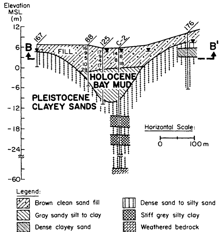
Figure 12. Cross-Section B-B' in the Mission District
