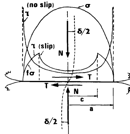
Fig. 2. Stress and strain on contact surface of two like spheres subjected to normal force N followed by a tangential force T
