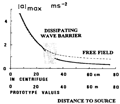
Fig. 8. Efficiency of the proposed dissipating wave barrier
