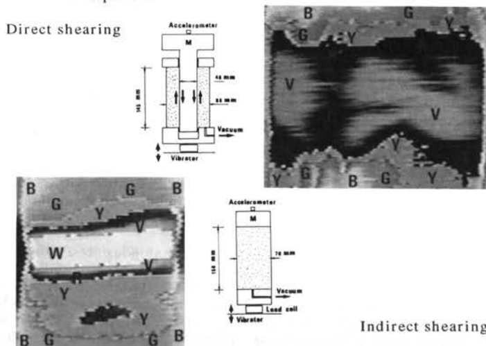
Fig. 4. Infrared thermography of the energy dissipation of a siliceous fine sand subjected to vibratory shearings (10 °C for each color hue)
