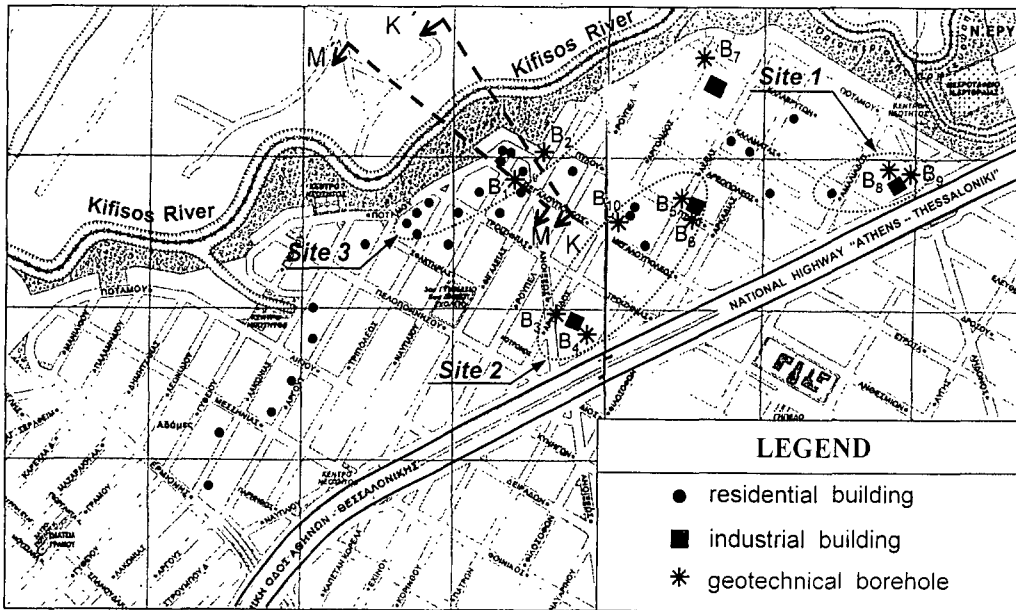
Figure 3 Plan view of Adames showing the heavily damaged and collapsed residential and industrial buildings. The location of the geotechnical boreholes (B 1 - B 10 ) and of the two topographic cross sections (K-K' & M-M') are also presented.
