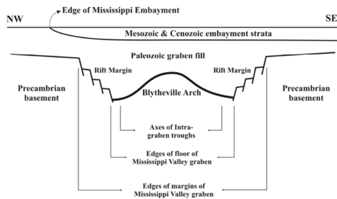
Figure 4. Northwest-Southeast cross-section of the Reelfoot Rift and Blytheville Arch (modified from McKeown and Diehl, 1994).
