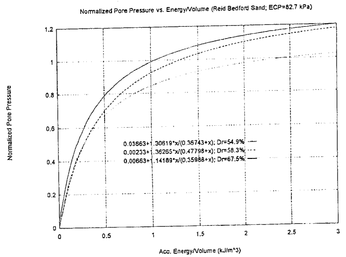
Figure 7. Hyperbolic Relationships for Reid Bedford Sand
