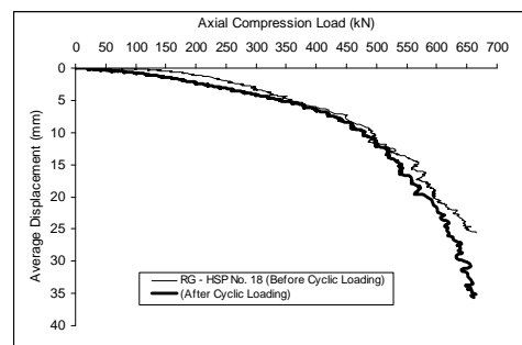
Fig.11. Load-displacement curves for RG-HSP 18 before and after cyclic loading
