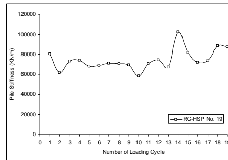
Fig.20. Stage 3 – RG-HSP 19 stiffness variation with number of loading cycles.
