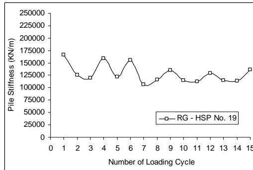
Fig. 14. RG-HSP 19 pile stiffness versus number of loading cycles
