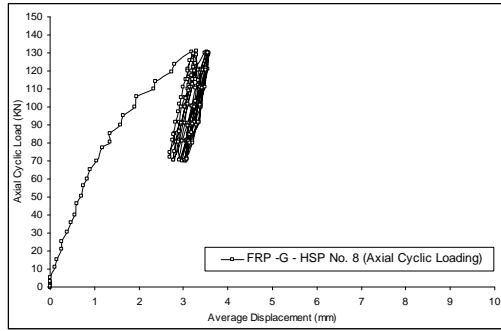
Fig. 13. FRP-G-HSP 8 axial cyclic load versus displacement
