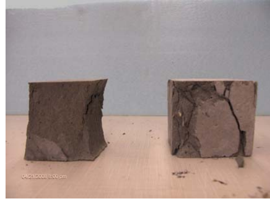
Fig.3. Compression strength test on the cubes without (left) and with steel fibres (right).
