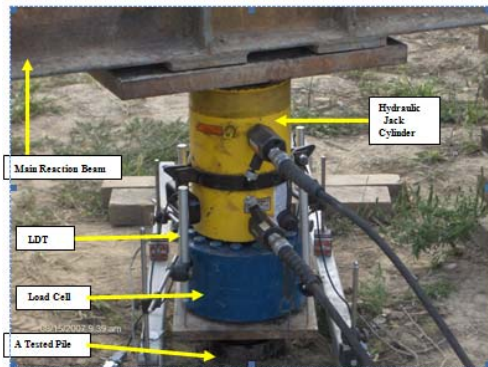
Fig.9. Hydraulic jack – load cell – loading plate – LDTs (axial compression loading setup)
