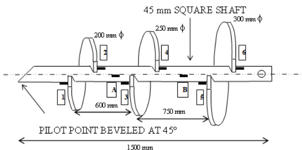
Fig.4. Schematic of lead section instrumentation with strain gauges
