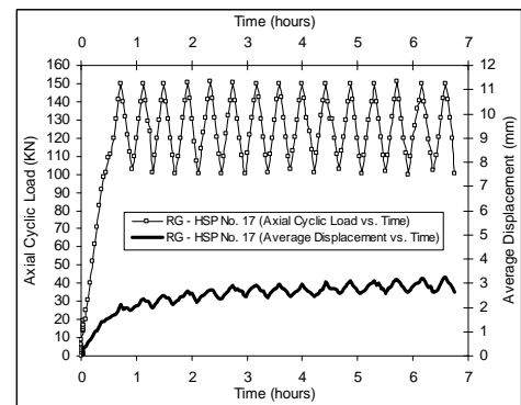
Fig.12. RG-HSP 17 axial cyclic load and displacement versus time
