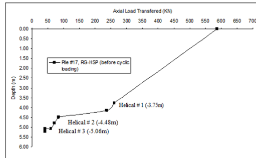
Fig. 15. RG-HSP 17 axial load transfer
