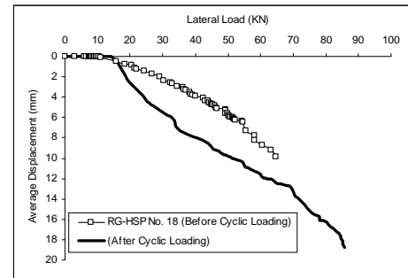
Fig.18. Stage 3 – RG-HSP 17 lateral load-displacement (before and after cyclic loading)
