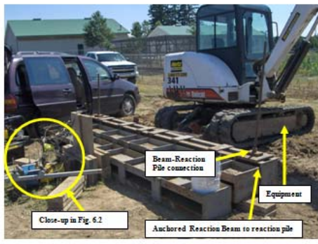
Fig.16. Lateral loading setup
