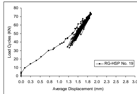
Fig.19. Stage 3 – RG-HSP 19 lateral cyclic load-displacement curve
