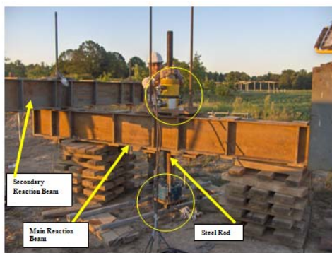
Fig.10. Axial cyclic loading setup
