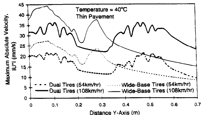
Fig. 6. Maximum particle velocity variation in transverse direction.
