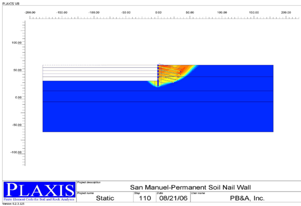
Figure 4: Global Stability Analysis by Phi-c reduction
