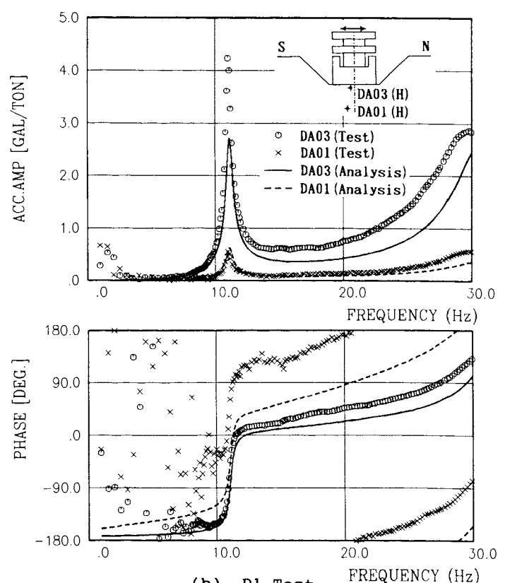
(a) C1 Test FREQUENCY (Hz) (b) D1 Test FREQUENCY (Hz) Fig.13 Comparison of Analysis and Test on Resonance Curves and Phase Lag Curves of Supporting Ground
