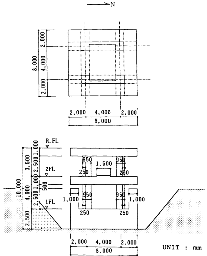
Fig.2 Shape of Model
