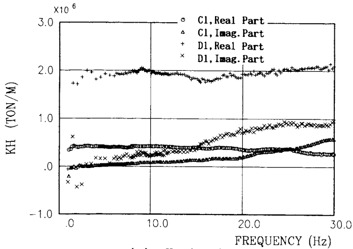
(a) Horizontal ( K_H ) (b) Rotational ( K_R ) Fig.5 Soil Impedances ( K_H , K_R ) at Base Bottom
