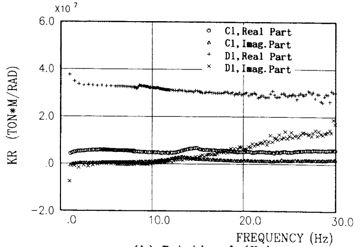
(a) Horizontal ( K_H ) (b) Rotational ( K_R ) Fig.5 Soil Impedances ( K_H , K_R ) at Base Bottom
