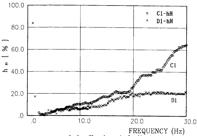
(a) Horizontal ( h_H ) (b) Rotational ( h_R ) Fig.6 Equivalent Damping Factors ( h = \text{Imag.} / (2 \times \text{Real}) )
