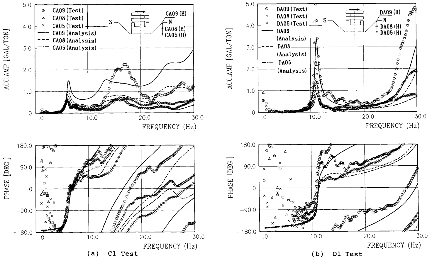
(a) C1 Test (b) D1 Test Fig.14 Comparison of Analysis and Test on Resonance Curves and Phase Lag Curves of Surrounding Ground
