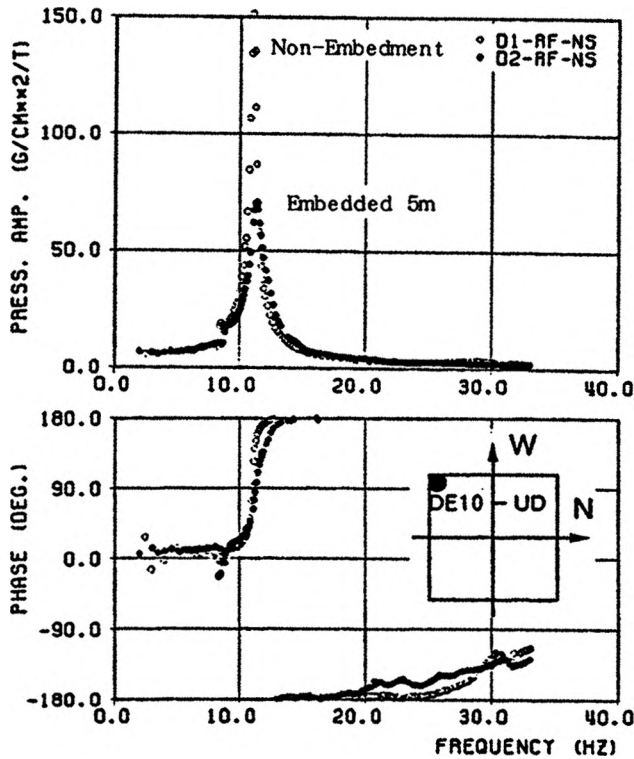
Fig. 9 Resonance Curves of Soil Pressure (Comparison between D1 and D2)
