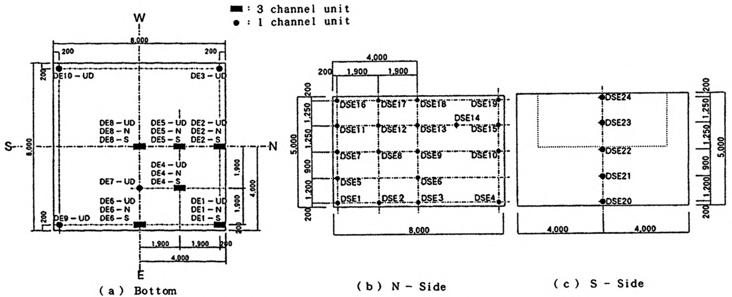
Fig. 4 Location of Soil Pressure Measuring Points
