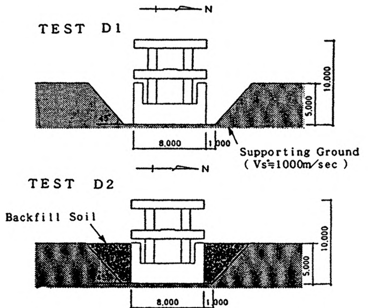
Fig. 1 D-Test Models
