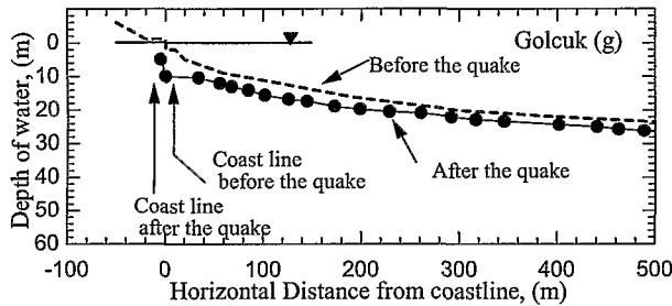
Fig. 9. Result of Measurement of water depth (Golcuk)
