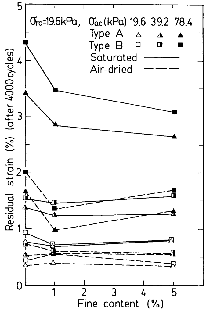
Fig.7 Residual Strain after 4000 Cycles versus Fine Content
