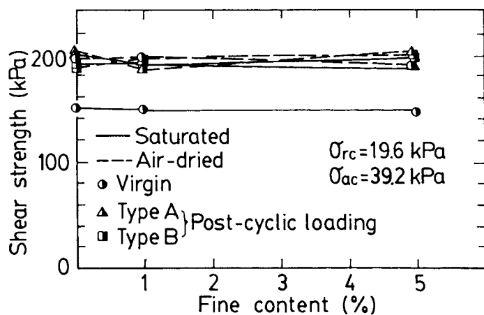
Fig. 10 Shear Strength versus Fine Content
