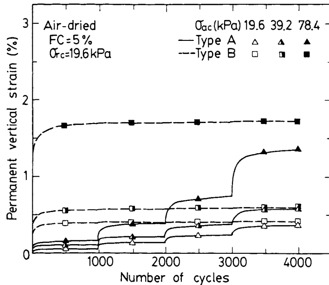
Fig.4 Permanent Vertical Strains versus Number of Cycles of Air-Dried Samples (FC = 5 %)
