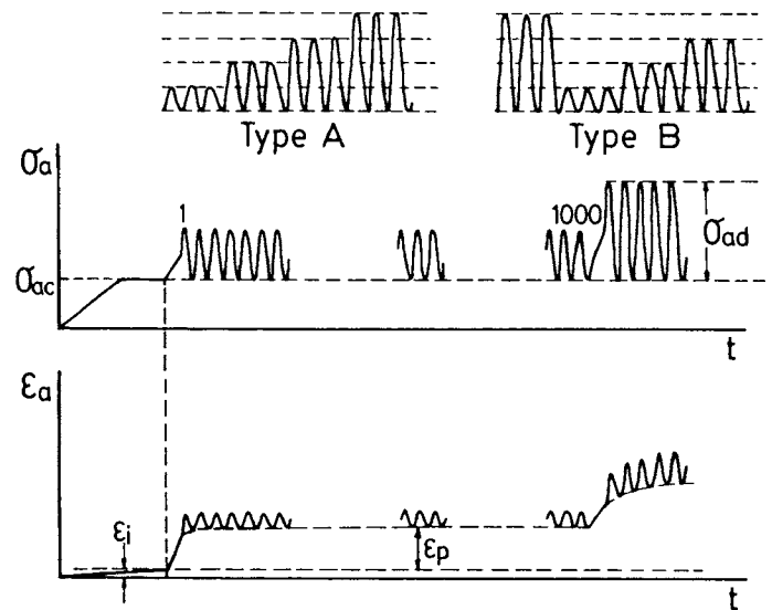
Fig.2 Schematic Illustration of Cyclic Loading
