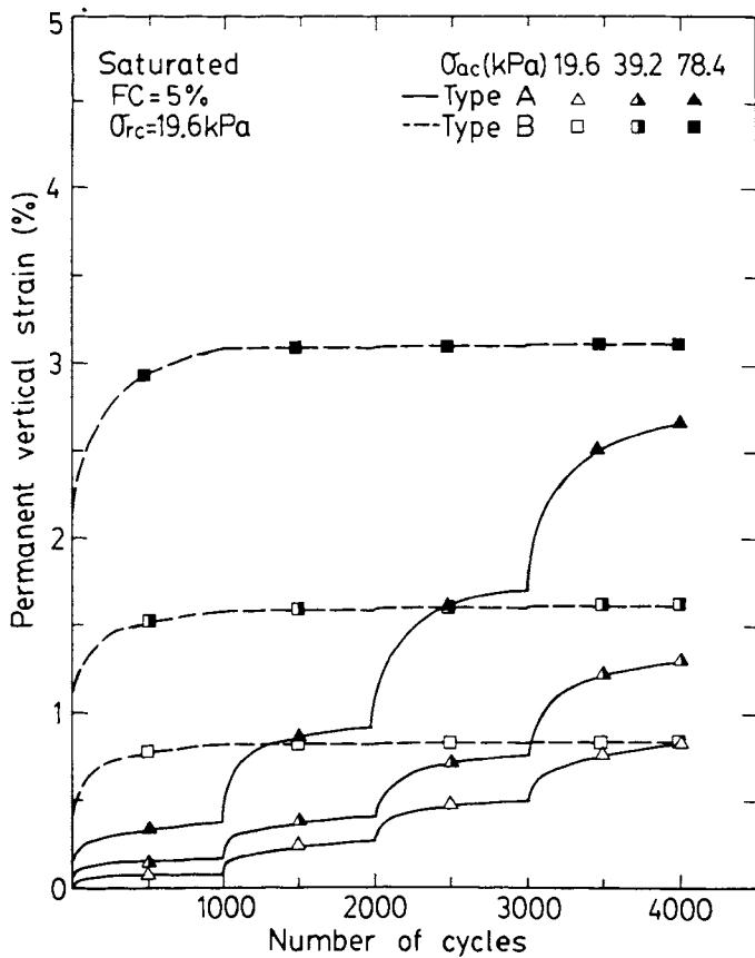
Fig.6 Permanent Vertical Strains versus Number of Cycles of Saturated Samples (FC = 5 %)
