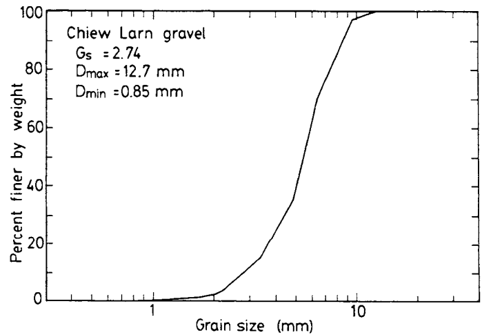
Fig.1 Grain Size Distribution of Coarse Material
