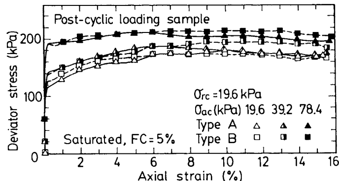
Fig. 9 Stress-Strain Curves of Saturated Post-Cyclic Loading Samples (FC = 5 %)
