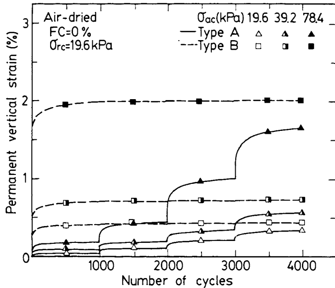
Fig.3 Permanent Vertical Strains versus Number of Cycles of Air-Dried Samples (FC = 0 %)
