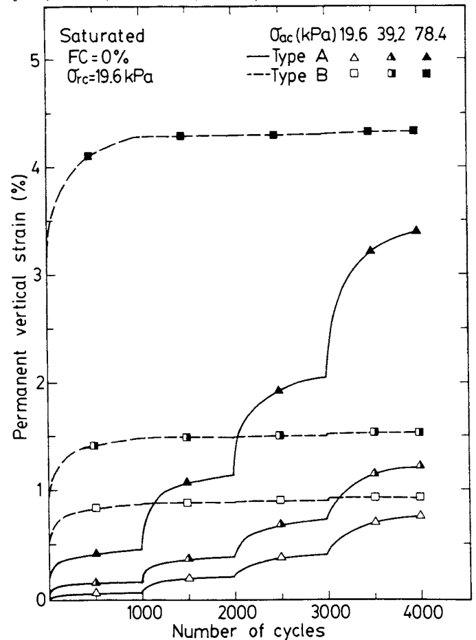
Fig.5 Permanent Vertical Strains versus Number of Cycles of Saturated Samples (FC = 0 %)
