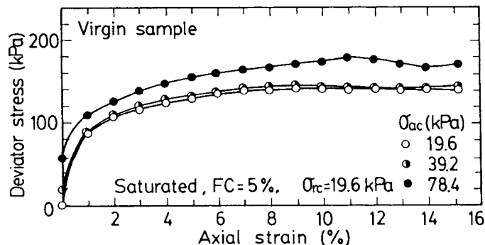
Fig. 8 Stress-Strain Curves of Saturated Virgin Samples (FC = 5 %)
