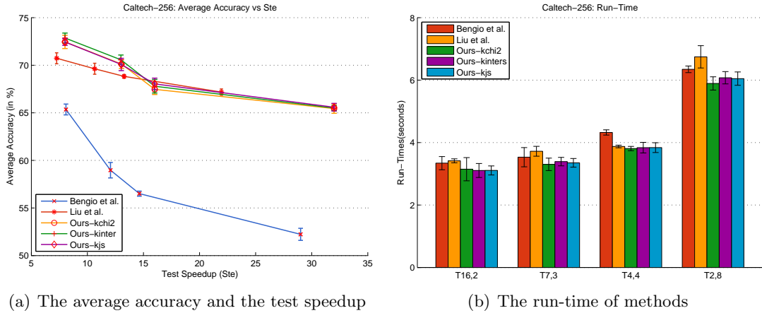
Figure 6. Performance of the evaluated methods using the CNN feature on Caltech-256
