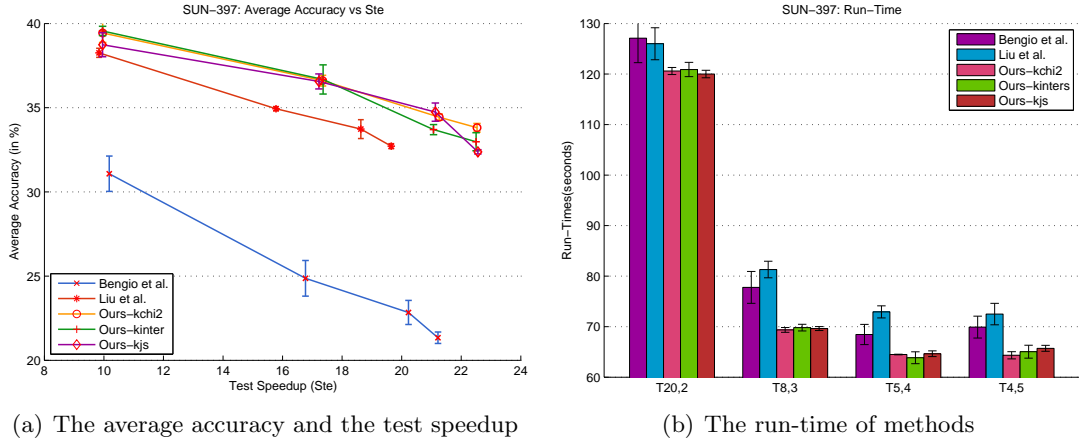
Figure 3. Performance of the evaluated methods using the SIFT+LLC+SPM feature on SUN-397
