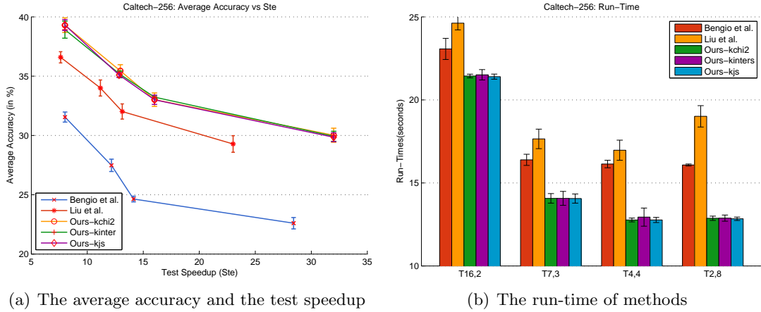
Figure 5. Performance of methods using the SIFT+LLC+SPM feature on Caltech-256
