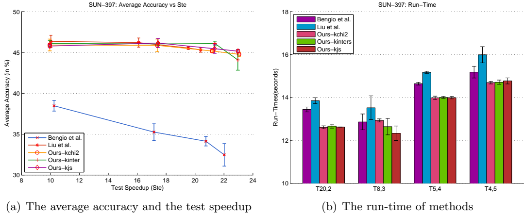
Figure 4. Performance of the evaluated methods using the CNN feature on SUN-397
