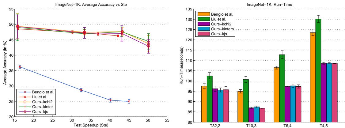
(a) The average accuracy and the test speedup
