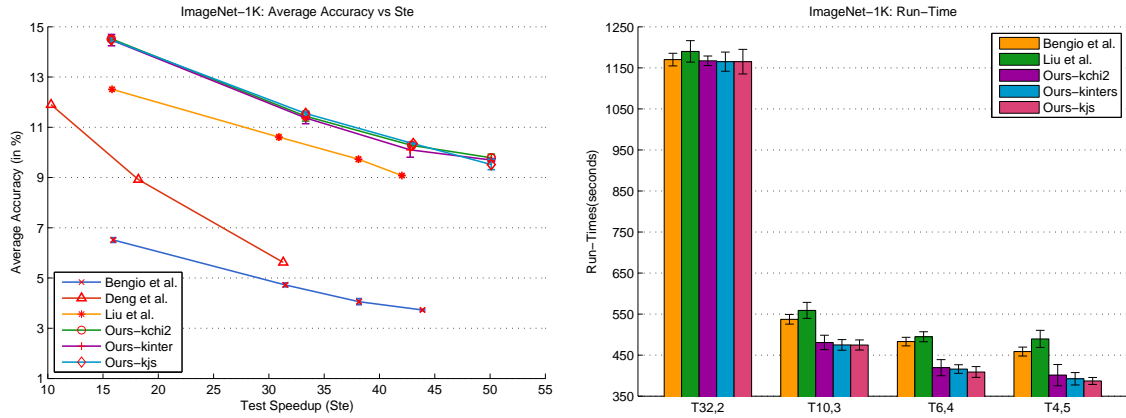
(a) The average accuracy and the test speedup of methods
