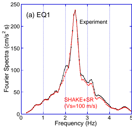
Fig. 12. Fourier amplitude spectrum of observed and computed superstructure acceleration.
