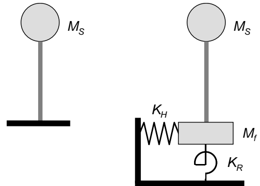
(a) Fixed footing model (b) SR-model
