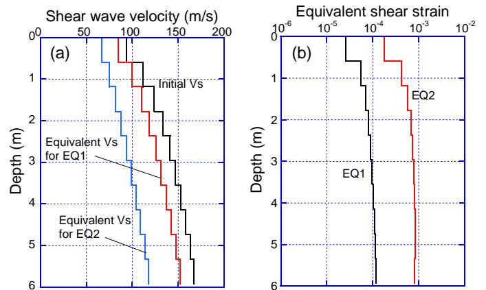
Fig. 8. Initial and equivalent V_s profiles and equivalent shear strain profiles.
